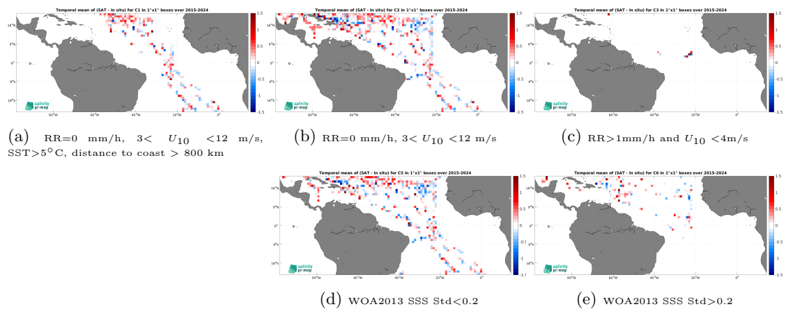
Figure 14: Temporal mean gridded over spatial boxes of size 1^\circ \times 1^\circ of \Delta\text{SSS} (SMAP SSS L2 v6 - 40 km (RSS) - TSG (SAMOS)) for 5 different subdatasets corresponding to:RR=0 mm/h, 3 < U_{10} < 12 m/s, SST > 5°C, distance to coast > 800 km (a), RR=0 mm/h, 3 < U_{10} < 12 m/s (b), RR > 1mm/h and U_{10} < 4 m/s (c), WOA2013 SSS Std < 0.2 (d), WOA2013 SSS Std > 0.2 (e).
