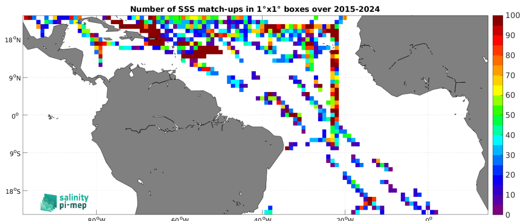
Figure 5: Number of SSS match-ups between TSG (SAMOS) SSS and the SMAP SSS L2 v6 - 40 km (RSS) SSS product for the Tropical Atlantic Ocean Pi-MEP region over 1^\circ \times 1^\circ boxes and for the full satellite product period.
