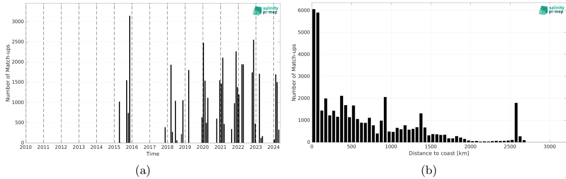
Figure 2: Number of match-ups between TSG (SAMOS) and SMAP SSS L2 v6 - 40 km (RSS) SSS as a function of time (a) and as function of the distance to coast (b) over the Tropical Atlantic Ocean Pi-MEP region and for the full satellite product period.
