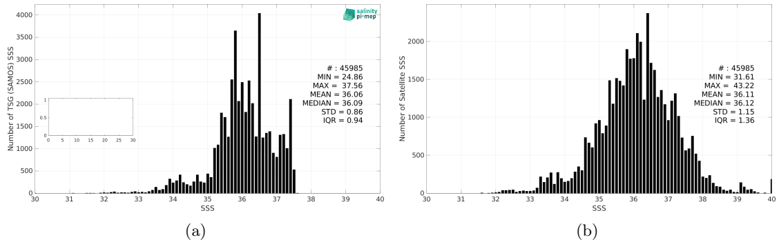
Figure 3: Histograms of SSS from TSG (SAMOS) (a) and SMAP SSS L2 v6 - 40 km (RSS) (b) considering all match-up pairs per bins of 0.1 over the Tropical Atlantic Ocean Pi-MEP region and for the full satellite product period.
