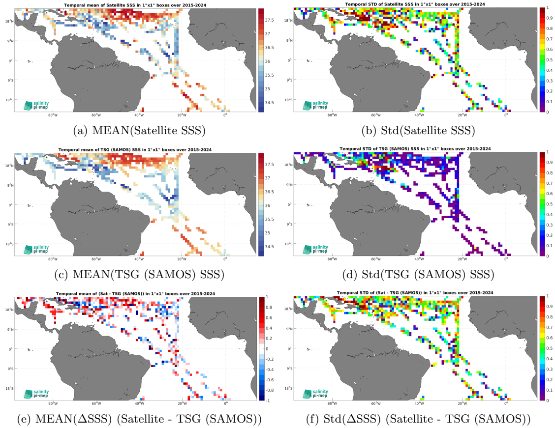
Figure 7: Temporal mean (left) and Std (right) of SSS from SMAP SSS L2 v6 - 40 km (RSS) (top), TSG (SAMOS) (middle), and of \Delta SSS (Satellite - TSG (SAMOS)). Only match-up pairs are used to generate these maps.
