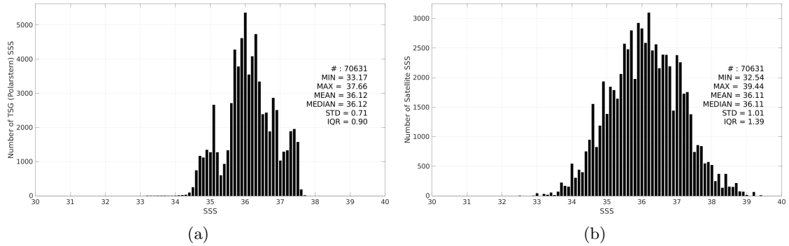
Figure 3: Histograms of SSS from TSG (Polarstern) (a) and SMAP SSS L2 v6 - 40 km (RSS) (b) considering all match-up pairs per bins of 0.1 over the Tropical Atlantic Ocean Pi-MEP region and for the full satellite product period.
