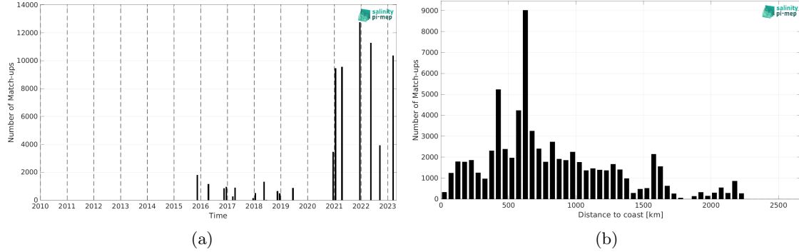
Figure 2: Number of match-ups between TSG (Polarstern) and SMAP SSS L2 v6 - 40 km (RSS) SSS as a function of time (a) and as function of the distance to coast (b) over the Tropical Atlantic Ocean Pi-MEP region and for the full satellite product period.
