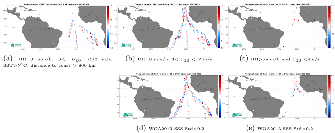
Figure 14: Temporal mean gridded over spatial boxes of size 1^\circ \times 1^\circ of \Delta SSS (SMAP SSS L2 v6 - 40 km (RSS) - TSG (Polarstern)) for 5 different subdatasets corresponding to: RR=0 mm/h, 3 < U_{10} < 12 m/s, SST > 5°C, distance to coast > 800 km (a), RR=0 mm/h, 3 < U_{10} < 12 m/s (b), RR > 1 mm/h and U_{10} < 4 m/s (c), WOA2013 SSS Std < 0.2 (d), WOA2013 SSS Std > 0.2 (e).
