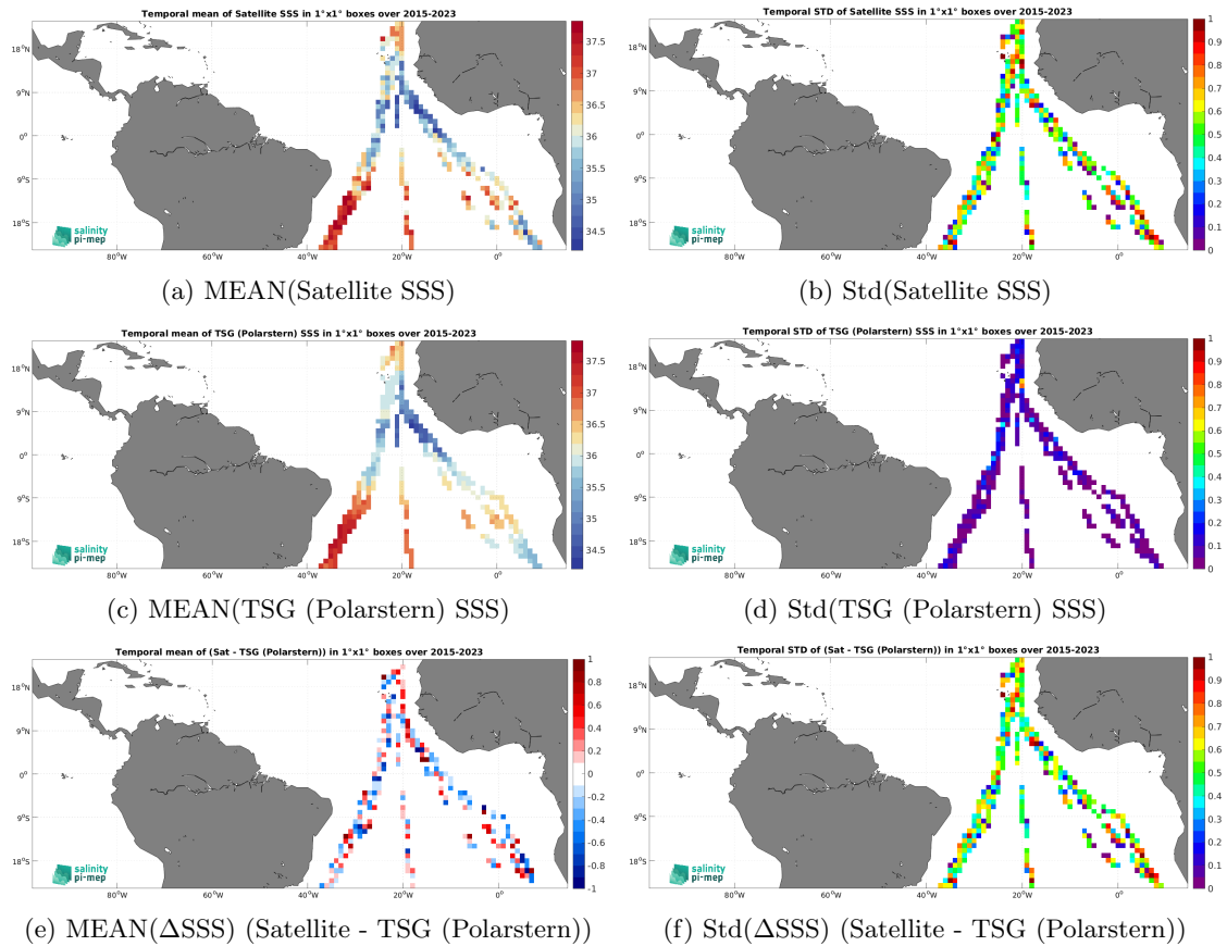
Figure 7: Temporal mean (left) and Std (right) of SSS from SMAP SSS L2 v6 - 40 km (RSS) (top), TSG (Polarstern) (middle), and of \Delta SSS (Satellite - TSG (Polarstern)). Only match-up pairs are used to generate these maps.
