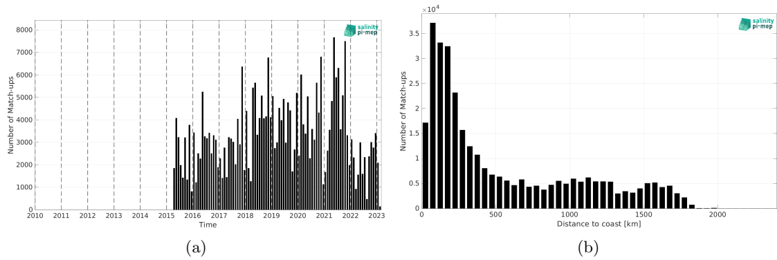
Figure 2: Number of match-ups between TSG (LEGOS-DM) and SMAP SSS L2 v6 - 40 km (RSS) SSS as a function of time (a) and as function of the distance to coast (b) over the Tropical Atlantic Ocean Pi-MEP region and for the full satellite product period.
