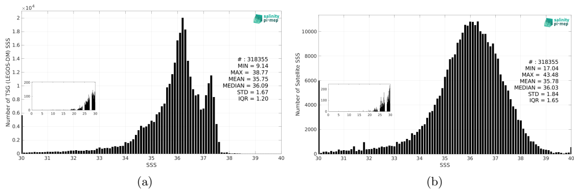
Figure 3: Histograms of SSS from TSG (LEGOS-DM) (a) and SMAP SSS L2 v6 - 40 km (RSS) (b) considering all match-up pairs per bins of 0.1 over the Tropical Atlantic Ocean Pi-MEP region and for the full satellite product period.
