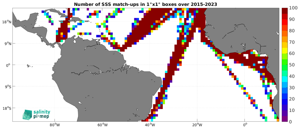
Figure 5: Number of SSS match-ups between TSG (LEGOS-DM) SSS and the SMAP SSS L2 v6 - 40 km (RSS) SSS product for the Tropical Atlantic Ocean Pi-MEP region over 1^\circ \times 1^\circ boxes and for the full satellite product period.
