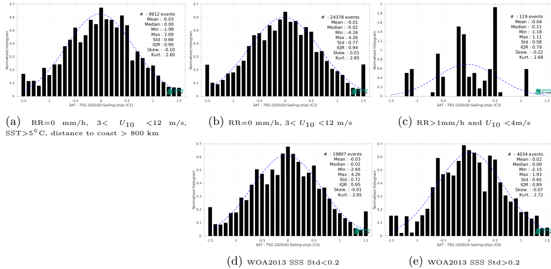
Figure 15: Normalized histogram of \Delta\text{SSS} (SMAP SSS L2 v6 - 40 km (RSS) - TSG (GOSUD-Sailing-ship)) for 5 different subdatasets corresponding to: RR=0 mm/h, 3 < U_{10} < 12 m/s, SST>5°C, distance to coast > 800 km (a), RR=0 mm/h, 3 < U_{10} < 12 m/s (b), RR>1mm/h and U_{10} < 4 m/s (c), WOA2013 SSS Std<0.2 (d), WOA2013 SSS Std>0.2 (e).
