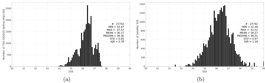
Figure 3: Histograms of SSS from TSG (GOSUD-Sailing-ship) (a) and SMAP SSS L2 v6 - 40 km (RSS) (b) considering all match-up pairs per bins of 0.1 over the Tropical Atlantic Ocean Pi-MEP region and for the full satellite product period.
