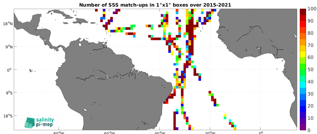
Figure 5: Number of SSS match-ups between TSG (GOSUD-Sailing-ship) SSS and the SMAP SSS L2 v6 - 40 km (RSS) SSS product for the Tropical Atlantic Ocean Pi-MEP region over 1^\circ \times 1^\circ boxes and for the full satellite product period.
