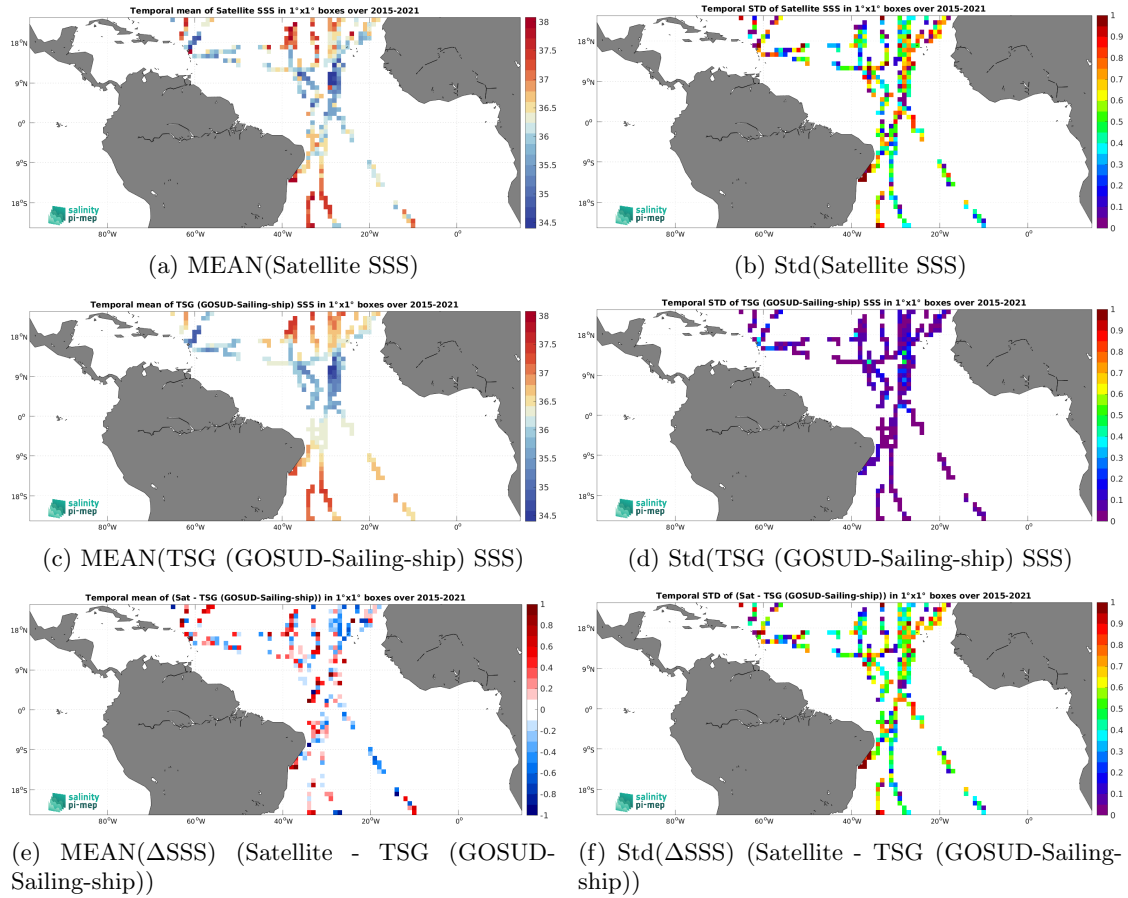
Figure 7: Temporal mean (left) and Std (right) of SSS from SMAP SSS L2 v6 - 40 km (RSS) (top), TSG (GOSUD-Sailing-ship) (middle), and of \Delta SSS (Satellite - TSG (GOSUD-Sailing-ship)). Only match-up pairs are used to generate these maps.
