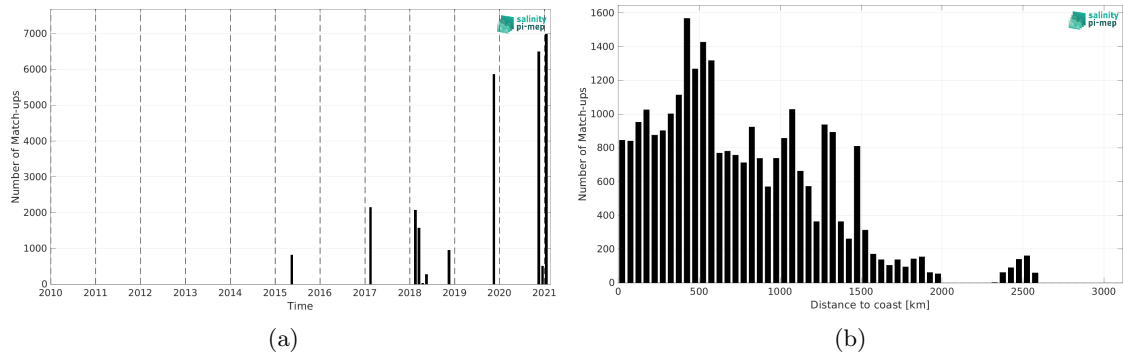
Figure 2: Number of match-ups between TSG (GOSUD-Sailing-ship) and SMAP SSS L2 v6 - 40 km (RSS) SSS as a function of time (a) and as function of the distance to coast (b) over the Tropical Atlantic Ocean Pi-MEP region and for the full satellite product period.
