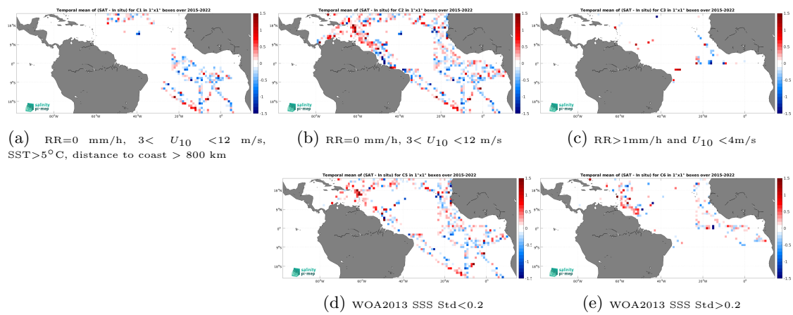
Figure 14: Temporal mean gridded over spatial boxes of size 1^\circ \times 1^\circ of \Delta\text{SSS} (SMAP SSS L2 v6 - 40 km (RSS) - TSG (GOSUD-Research-vessel)) for 5 different subdatasets corresponding to:RR=0 mm/h, 3 < U_{10} < 12 m/s, SST >5^\circ\text{C} , distance to coast > 800 km (a), RR=0 mm/h, 3 < U_{10} < 12 m/s (b), RR >1 mm/h and U_{10} < 4 m/s (c), WOA2013 SSS Std <0.2 (d), WOA2013 SSS Std >0.2 (e).
