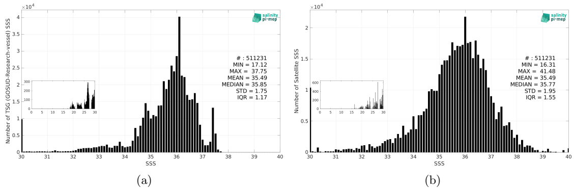
Figure 3: Histograms of SSS from TSG (GOSUD-Research-vessel) (a) and SMAP SSS L2 v6 - 40 km (RSS) (b) considering all match-up pairs per bins of 0.1 over the Tropical Atlantic Ocean Pi-MEP region and for the full satellite product period.
