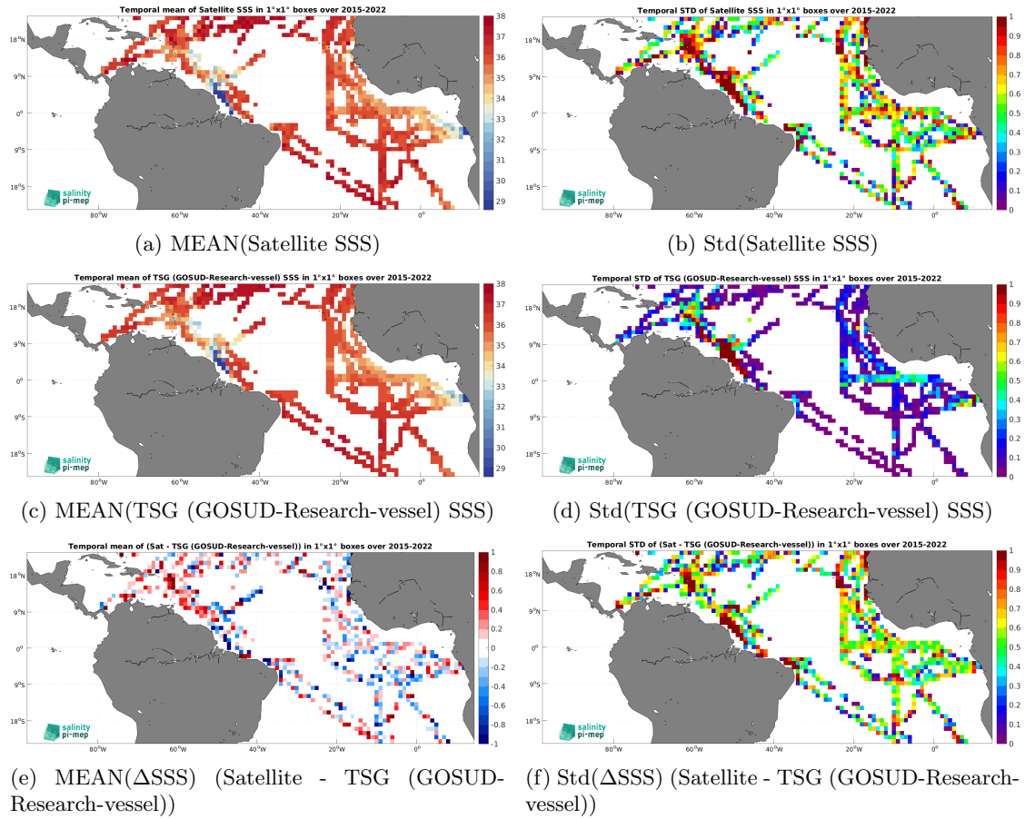
Figure 7: Temporal mean (left) and Std (right) of SSS from SMAP SSS L2 v6 - 40 km (RSS) (top), TSG (GOSUD-Research-vessel) (middle), and of \Delta SSS (Satellite - TSG (GOSUD-Research-vessel)). Only match-up pairs are used to generate these maps.
