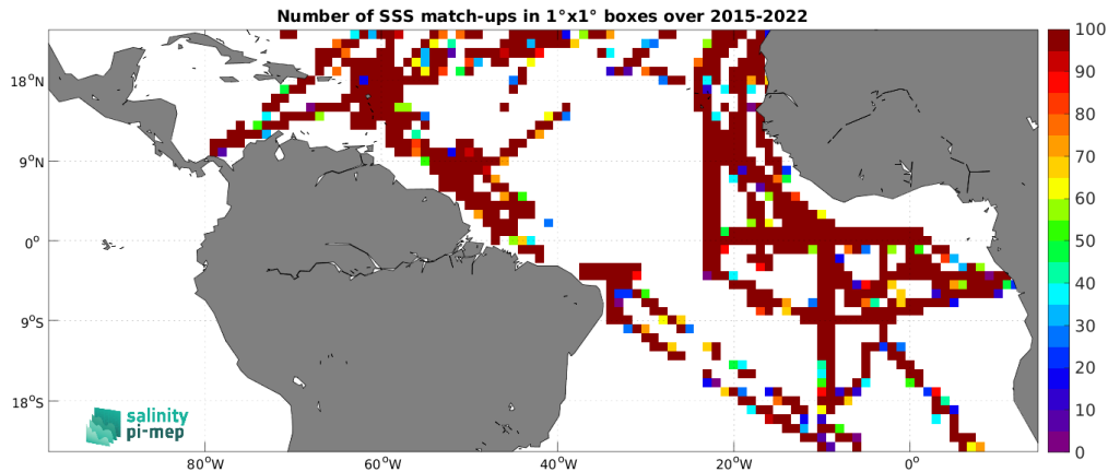
Figure 5: Number of SSS match-ups between TSG (GOSUD-Research-vessel) SSS and the SMAP SSS L2 v6 - 40 km (RSS) SSS product for the Tropical Atlantic Ocean Pi-MEP region over 1^\circ \times 1^\circ boxes and for the full satellite product period.
