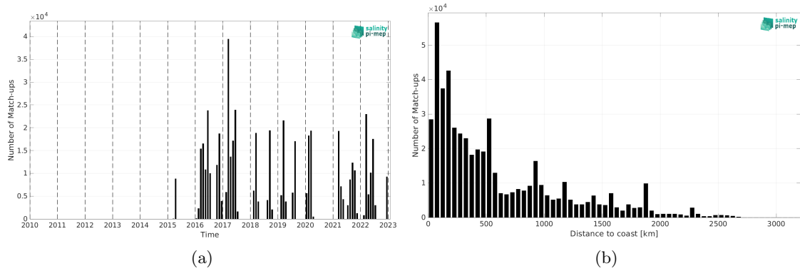
Figure 2: Number of match-ups between TSG (GOSUD-Research-vessel) and SMAP SSS L2 v6 - 40 km (RSS) SSS as a function of time (a) and as function of the distance to coast (b) over the Tropical Atlantic Ocean Pi-MEP region and for the full satellite product period.
