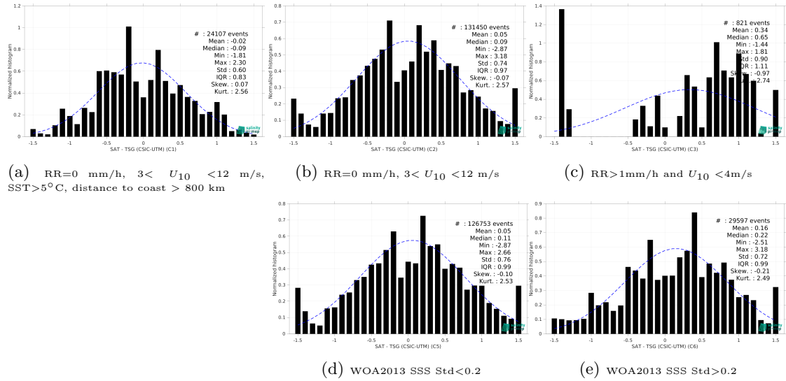
Figure 15: Normalized histogram of \Delta\text{SSS} (SMAP SSS L2 v6 - 40 km (RSS) - TSG (CSIC-UTM)) for 5 different subdatasets corresponding to: RR=0 mm/h, 3 < U_{10} < 12 m/s, SST > 5^\circ\text{C} , distance to coast > 800 km (a), RR=0 mm/h, 3 < U_{10} < 12 m/s (b), RR > 1 mm/h and U_{10} < 4 m/s (c), WOA2013 SSS Std < 0.2 (d), WOA2013 SSS Std > 0.2 (e).
