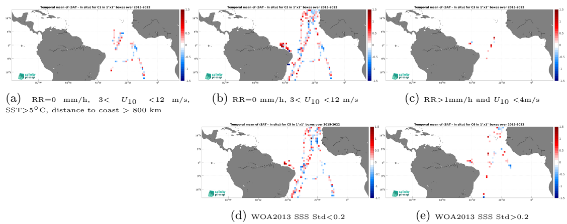
Figure 14: Temporal mean gridded over spatial boxes of size 1^\circ \times 1^\circ of \Delta SSS (SMAP SSS L2 v6 - 40 km (RSS) - TSG (CSIC-UTM)) for 5 different subdatasets corresponding to:RR=0 mm/h, 3 < U_{10} < 12 m/s, SST >5^\circ\text{C} , distance to coast > 800 km (a), RR=0 mm/h, 3 < U_{10} < 12 m/s (b), RR >1 mm/h and U_{10} < 4 m/s (c), WOA2013 SSS Std <0.2 (d), WOA2013 SSS Std >0.2 (e).
