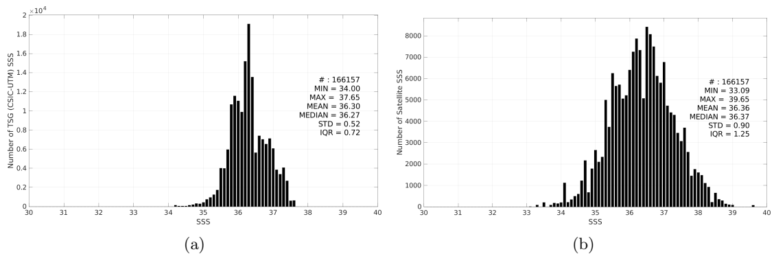
Figure 3: Histograms of SSS from TSG (CSIC-UTM) (a) and SMAP SSS L2 v6 - 40 km (RSS) (b) considering all match-up pairs per bins of 0.1 over the Tropical Atlantic Ocean Pi-MEP region and for the full satellite product period.
