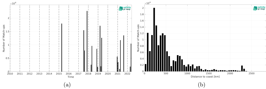
Figure 2: Number of match-ups between TSG (CSIC-UTM) and SMAP SSS L2 v6 - 40 km (RSS) SSS as a function of time (a) and as function of the distance to coast (b) over the Tropical Atlantic Ocean Pi-MEP region and for the full satellite product period.
