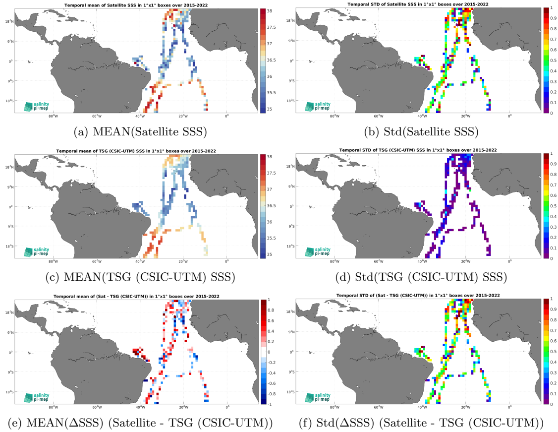
Figure 7: Temporal mean (left) and Std (right) of SSS from SMAP SSS L2 v6 - 40 km (RSS) (top), TSG (CSIC-UTM) (middle), and of \Delta SSS (Satellite - TSG (CSIC-UTM)). Only match-up pairs are used to generate these maps.
