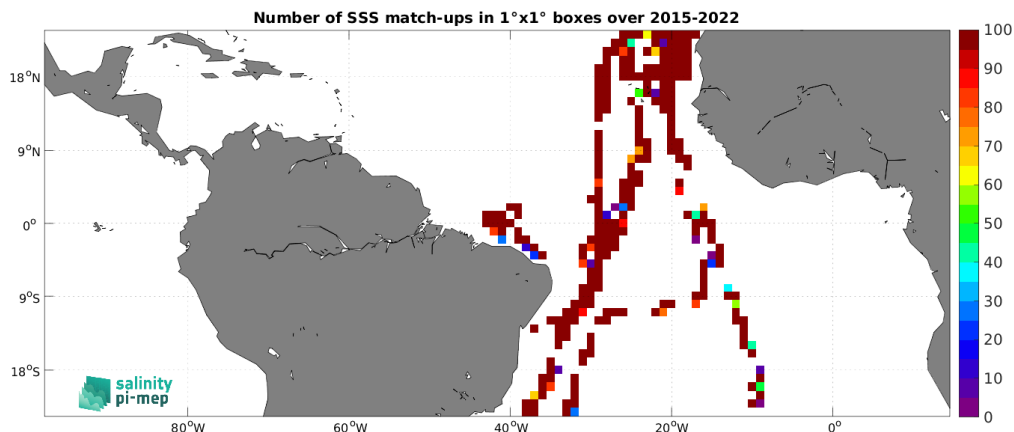
Figure 5: Number of SSS match-ups between TSG (CSIC-UTM) SSS and the SMAP SSS L2 v6 - 40 km (RSS) SSS product for the Tropical Atlantic Ocean Pi-MEP region over 1^\circ \times 1^\circ boxes and for the full satellite product period.
