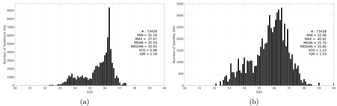
Figure 3: Histograms of SSS from Saildrone (a) and SMAP SSS L2 v6 - 40 km (RSS) (b) considering all match-up pairs per bins of 0.1 over the Tropical Atlantic Ocean Pi-MEP region and for the full satellite product period.
