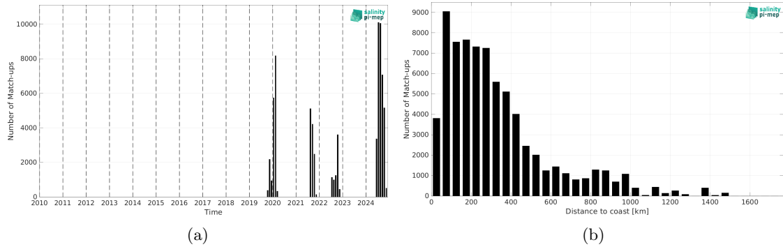
Figure 2: Number of match-ups between Saildrone and SMAP SSS L2 v6 - 40 km (RSS) SSS as a function of time (a) and as function of the distance to coast (b) over the Tropical Atlantic Ocean Pi-MEP region and for the full satellite product period.
