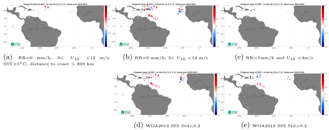
Figure 14: Temporal mean gridded over spatial boxes of size 1^\circ \times 1^\circ of \Delta\text{SSS} (SMAP SSS L2 v6 - 40 km (RSS) - Saldrone) for 5 different subdatasets corresponding to:RR=0 mm/h, 3 < U_{10} < 12 m/s, SST >5^\circ\text{C} , distance to coast > 800 km (a), RR=0 mm/h, 3 < U_{10} < 12 m/s (b), RR >1 mm/h and U_{10} < 4 m/s (c), WOA2013 SSS Std <0.2 (d), WOA2013 SSS Std >0.2 (e).
