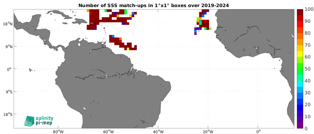
Figure 5: Number of SSS match-ups between Saildrone SSS and the SMAP SSS L2 v6 - 40 km (RSS) SSS product for the Tropical Atlantic Ocean Pi-MEP region over 1^\circ \times 1^\circ boxes and for the full satellite product period.
