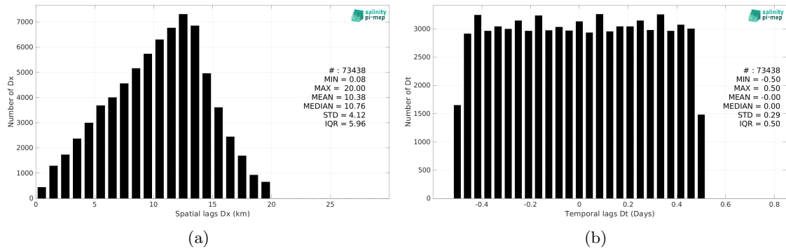
Figure 6: Histograms of the spatial (a) and temporal (b) lags between the location/time of the Saifdrone measurement and the date of the corresponding SMAP SSS L2 v6 - 40 km (RSS) SSS pixel.
