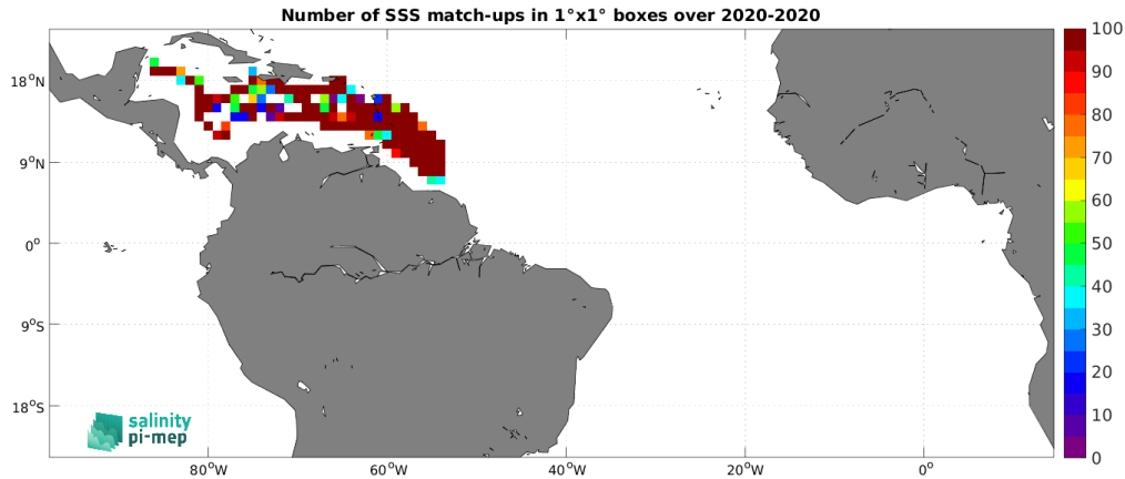
Figure 4: Number of SSS match-ups between Surface drifters SSS and the SMAP SSS L2 v6 - 40 km (RSS) SSS product for the Tropical Atlantic Ocean Pi-MEP region over 1^\circ \times 1^\circ boxes and for the full satellite product period.
