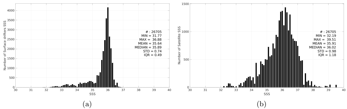
Figure 3: Histograms of SSS from Surface drifters (a) and SMAP SSS L2 v6 - 40 km (RSS) (b) considering all match-up pairs per bins of 0.1 over the Tropical Atlantic Ocean Pi-MEP region and for the full satellite product period.
