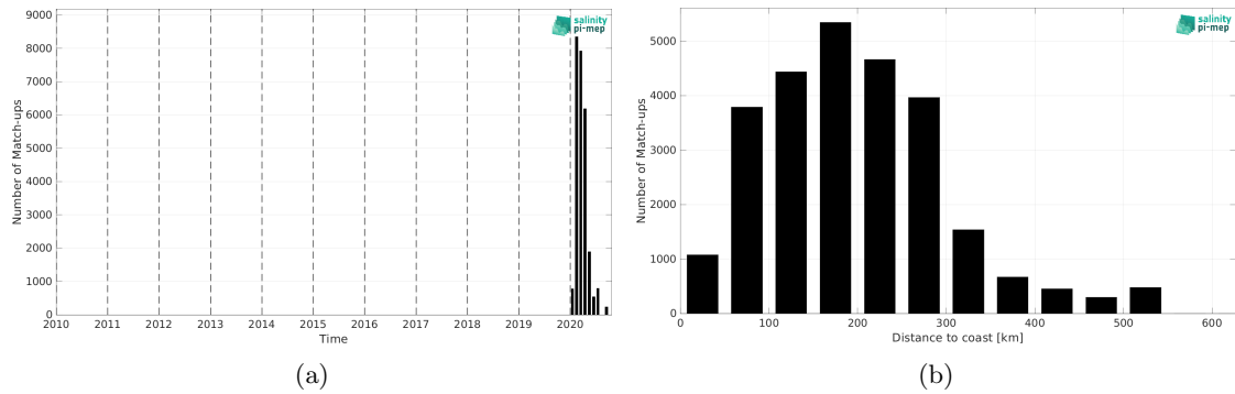
Figure 2: Number of match-ups between Surface drifters and SMAP SSS L2 v6 - 40 km (RSS) SSS as a function of time (a) and as function of the distance to coast (b) over the Tropical Atlantic Ocean Pi-MEP region and for the full satellite product period.
