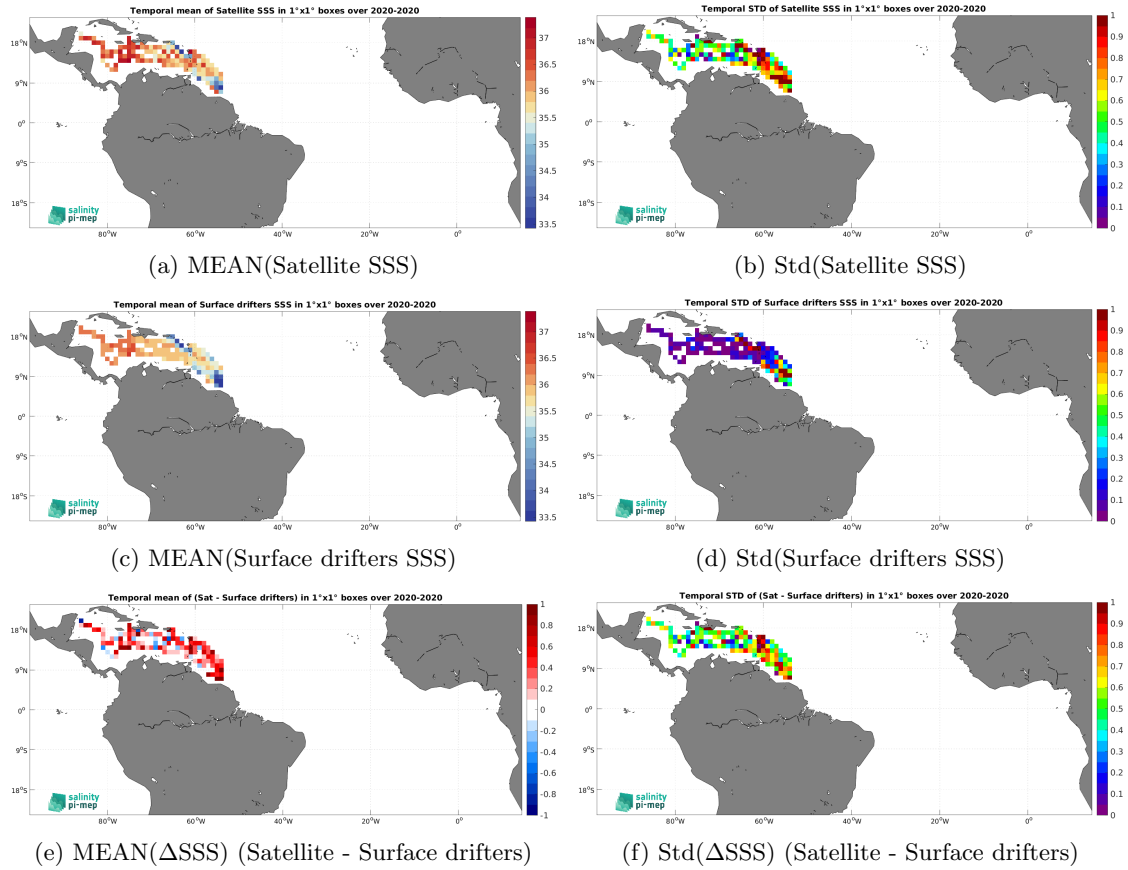
Figure 6: Temporal mean (left) and Std (right) of SSS from SMAP SSS L2 v6 - 40 km (RSS) (top), Surface drifters (middle), and of \Delta SSS (Satellite - Surface drifters). Only match-up pairs are used to generate these maps.
