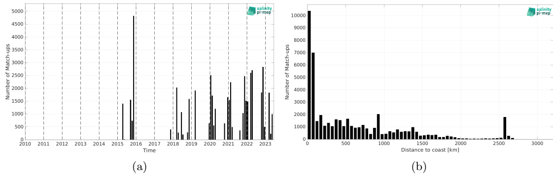
Figure 1: Number of match-ups between TSG (SAMOS) and SMAP SSS L2 v5 (RSS) SSS as a function of time (a) and as function of the distance to coast (b) over the Tropical Atlantic Ocean Pi-MEP region and for the full satellite product period.
