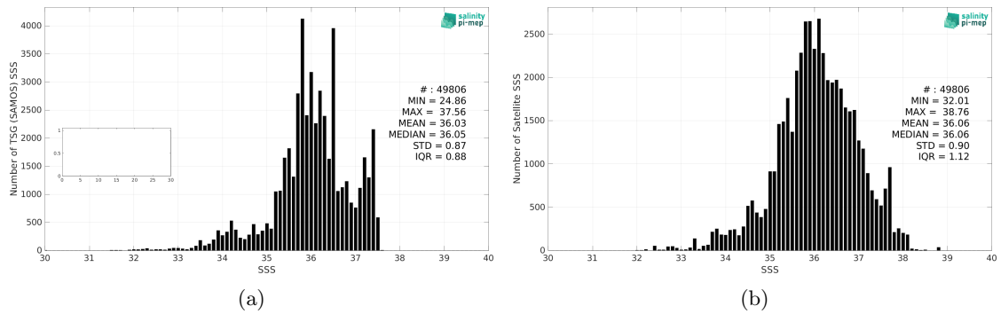
Figure 2: Histograms of SSS from TSG (SAMOS) (a) and SMAP SSS L2 v5 (RSS) (b) considering all match-up pairs per bins of 0.1 over the Tropical Atlantic Ocean Pi-MEP region and for the full satellite product period.
