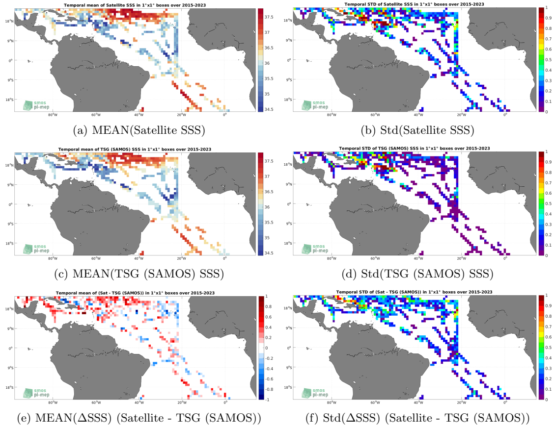
Figure 6: Temporal mean (left) and Std (right) of SSS from SMAP SSS L2 v5 (RSS) (top), TSG (SAMOS) (middle), and of \Delta SSS (Satellite - TSG (SAMOS)). Only match-up pairs are used to generate these maps.
