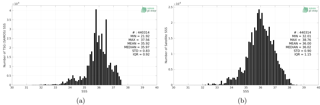
Figure 2: Histograms of SSS from TSG (SAMOS) (a) and SMAP SSS L2 v5 (RSS) (b) considering all match-up pairs per bins of 0.1 over the Tropical Atlantic Ocean Pi-MEP region and for the full satellite product period.
