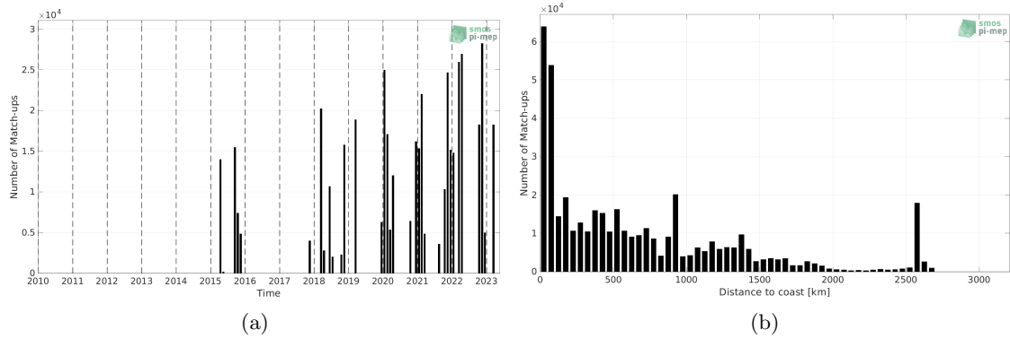
Figure 1: Number of match-ups between TSG (SAMOS) and SMAP SSS L2 v5 (RSS) SSS as a function of time (a) and as function of the distance to coast (b) over the Tropical Atlantic Ocean Pi-MEP region and for the full satellite product period.
