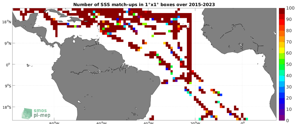
Figure 4: Number of SSS match-ups between TSG (SAMOS) SSS and the SMAP SSS L2 v5 (RSS) SSS product for the Tropical Atlantic Ocean Pi-MEP region over 1^\circ \times 1^\circ boxes and for the full satellite product period.
