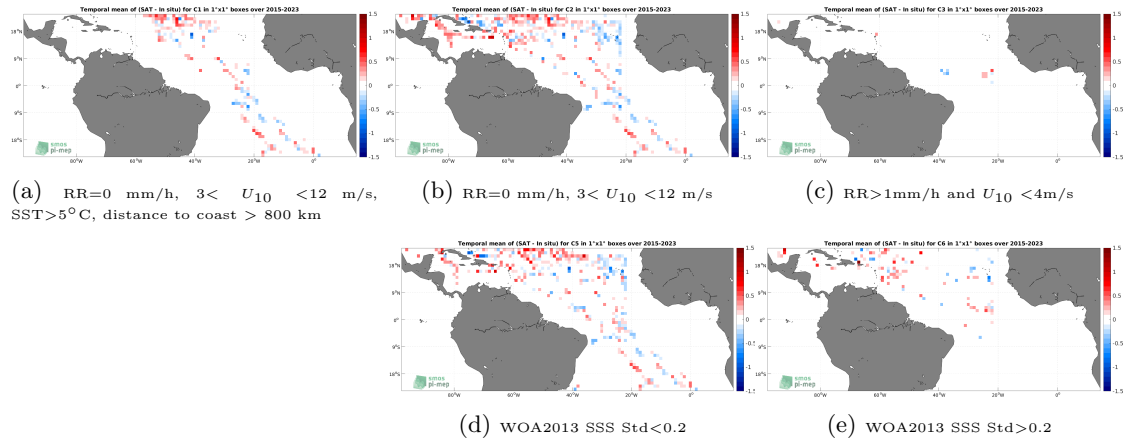
Figure 12: Temporal mean gridded over spatial boxes of size 1^\circ \times 1^\circ of \Delta\text{SSS} (SMAP SSS L2 v5 (RSS) - TSG (SAMOS)) for 5 different subdatasets corresponding to:RR=0 mm/h, 3 < U_{10} < 12 m/s, SST >5^\circ\text{C} , distance to coast > 800 km (a), RR=0 mm/h, 3 < U_{10} < 12 m/s (b), RR >1 mm/h and U_{10} < 4 m/s (c), WOA2013 SSS Std <0.2 (d), WOA2013 SSS Std >0.2 (e).
