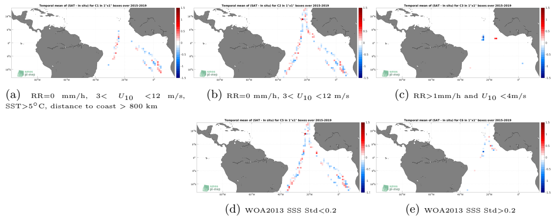
Figure 12: Temporal mean gridded over spatial boxes of size 1^\circ \times 1^\circ of \Delta\text{SSS} (SMAP SSS L2 v5 (RSS) - TSG (Polarstern)) for 5 different subdatasets corresponding to:RR=0 mm/h, 3 < U_{10} < 12 m/s, SST >5^\circ\text{C} , distance to coast > 800 km (a), RR=0 mm/h, 3 < U_{10} < 12 m/s (b), RR >1 mm/h and U_{10} < 4 m/s (c), WOA2013 SSS Std <0.2 (d), WOA2013 SSS Std >0.2 (e).
