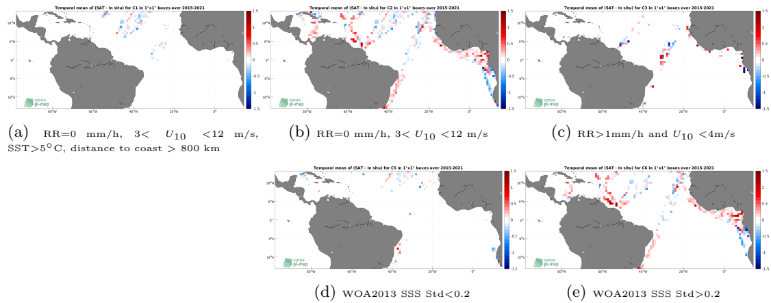
Figure 12: Temporal mean gridded over spatial boxes of size 1^\circ \times 1^\circ of \Delta\text{SSS} (SMAP SSS L2 v5 (RSS) - TSG (LEGOS-DM)) for 5 different subdatasets corresponding to:RR=0 mm/h, 3 < U_{10} < 12 m/s, SST >5^\circ\text{C} , distance to coast > 800 km (a), RR=0 mm/h, 3 < U_{10} < 12 m/s (b), RR >1 mm/h and U_{10} < 4 m/s (c), WOA2013 SSS Std <0.2 (d), WOA2013 SSS Std >0.2 (e).
