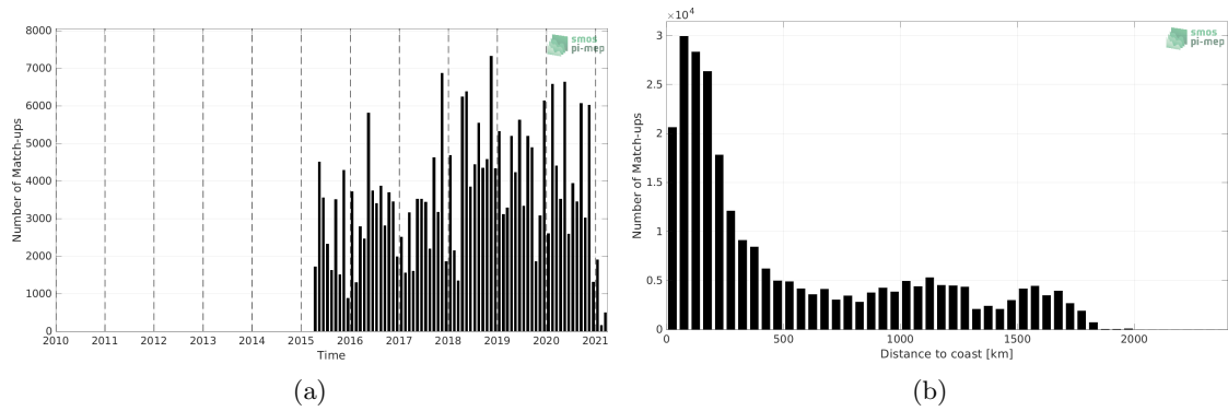
Figure 1: Number of match-ups between TSG (LEGOS-DM) and SMAP SSS L2 v5 (RSS) SSS as a function of time (a) and as function of the distance to coast (b) over the Tropical Atlantic Ocean Pi-MEP region and for the full satellite product period.
