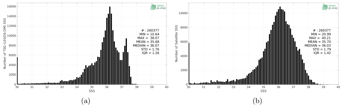
Figure 2: Histograms of SSS from TSG (LEGOS-DM) (a) and SMAP SSS L2 v5 (RSS) (b) considering all match-up pairs per bins of 0.1 over the Tropical Atlantic Ocean Pi-MEP region and for the full satellite product period.
