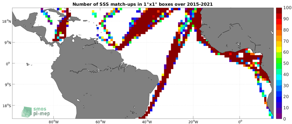
Figure 4: Number of SSS match-ups between TSG (LEGOS-DM) SSS and the SMAP SSS L2 v5 (RSS) SSS product for the Tropical Atlantic Ocean Pi-MEP region over 1^\circ \times 1^\circ boxes and for the full satellite product period.
