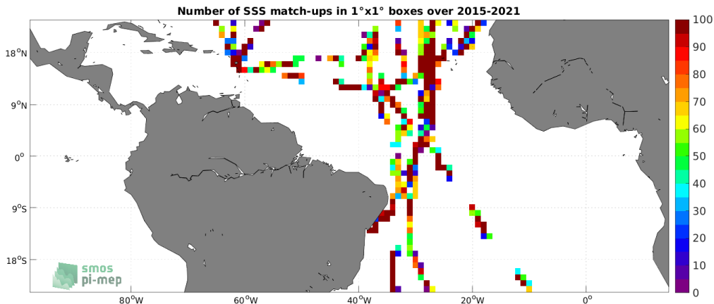
Figure 4: Number of SSS match-ups between TSG (GOSUD-Sailing-ship) SSS and the SMAP SSS L2 v5 (RSS) SSS product for the Tropical Atlantic Ocean Pi-MEP region over 1^\circ \times 1^\circ boxes and for the full satellite product period.
