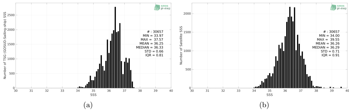
Figure 2: Histograms of SSS from TSG (GOSUD-Sailing-ship) (a) and SMAP SSS L2 v5 (RSS) (b) considering all match-up pairs per bins of 0.1 over the Tropical Atlantic Ocean Pi-MEP region and for the full satellite product period.
