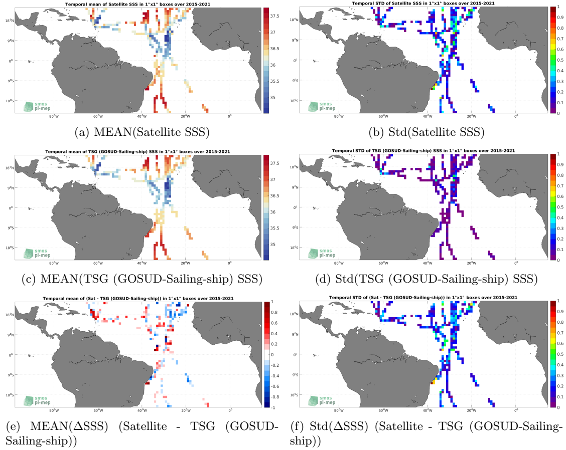
Figure 6: Temporal mean (left) and Std (right) of SSS from SMAP SSS L2 v5 (RSS) (top), TSG (GOSUD-Sailing-ship) (middle), and of \Delta SSS (Satellite - TSG (GOSUD-Sailing-ship)). Only match-up pairs are used to generate these maps.
