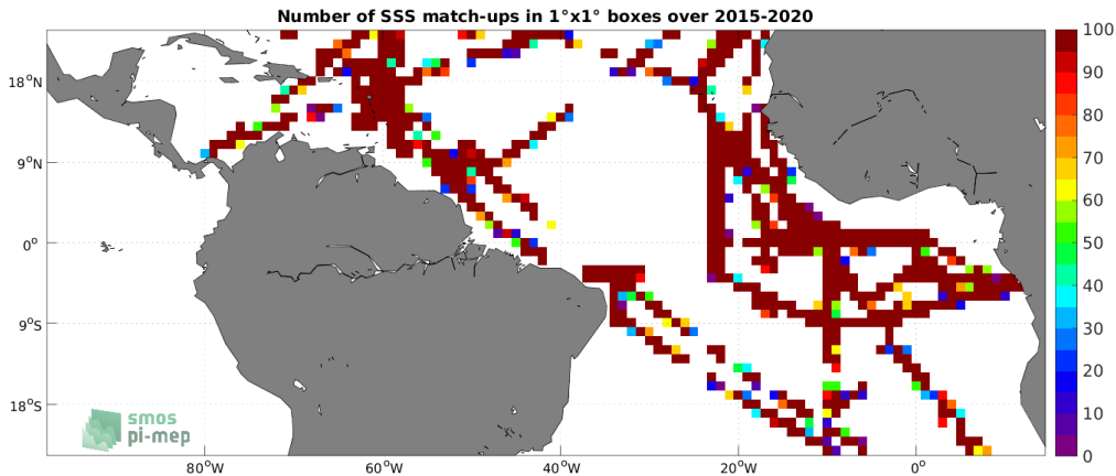
Figure 4: Number of SSS match-ups between TSG (GOSUD-Research-vessel) SSS and the SMAP SSS L2 v5 (RSS) SSS product for the Tropical Atlantic Ocean Pi-MEP region over 1^\circ \times 1^\circ boxes and for the full satellite product period.
