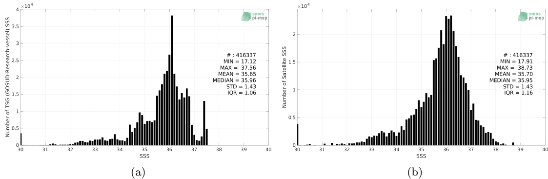
Figure 2: Histograms of SSS from TSG (GOSUD-Research-vessel) (a) and SMAP SSS L2 v5 (RSS) (b) considering all match-up pairs per bins of 0.1 over the Tropical Atlantic Ocean Pi-MEP region and for the full satellite product period.
