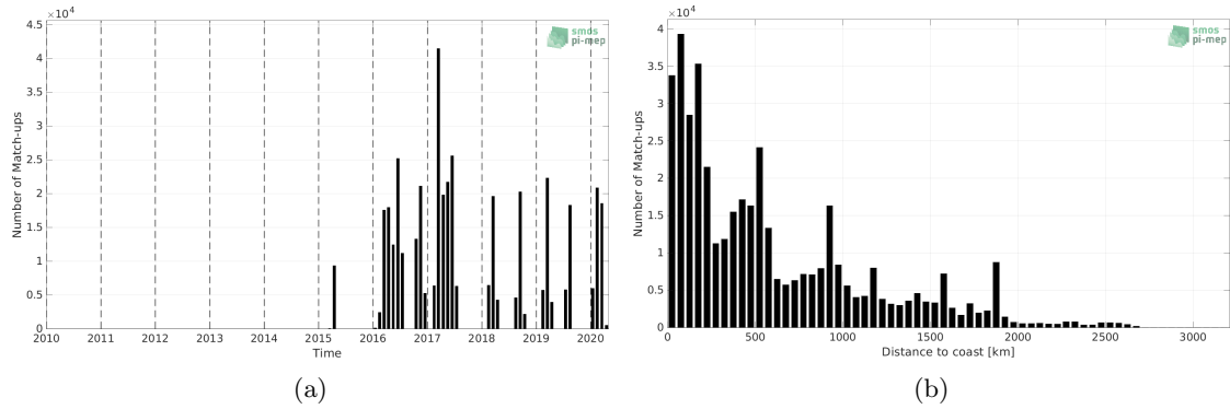
Figure 1: Number of match-ups between TSG (GOSUD-Research-vessel) and SMAP SSS L2 v5 (RSS) SSS as a function of time (a) and as function of the distance to coast (b) over the Tropical Atlantic Ocean Pi-MEP region and for the full satellite product period.
