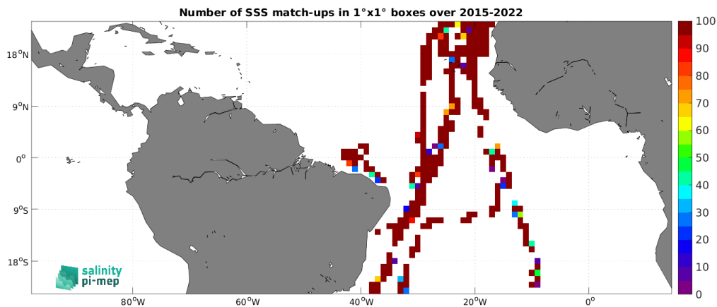
Figure 4: Number of SSS match-ups between TSG (CSIC-UTM) SSS and the SMAP SSS L2 v5 (RSS) SSS product for the Tropical Atlantic Ocean Pi-MEP region over 1^\circ \times 1^\circ boxes and for the full satellite product period.
