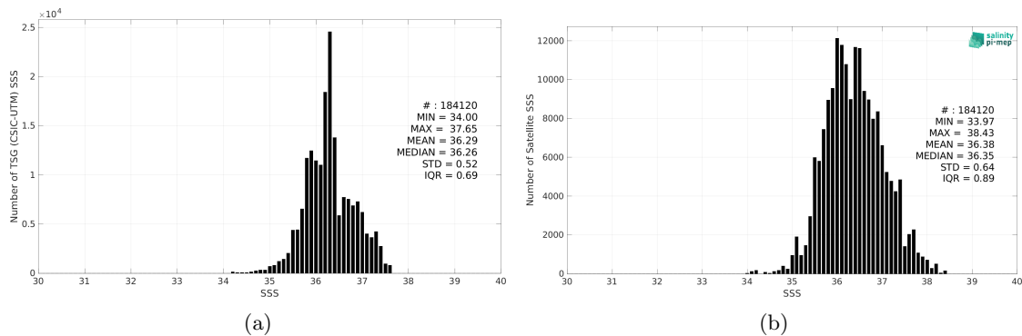
Figure 2: Histograms of SSS from TSG (CSIC-UTM) (a) and SMAP SSS L2 v5 (RSS) (b) considering all match-up pairs per bins of 0.1 over the Tropical Atlantic Ocean Pi-MEP region and for the full satellite product period.
