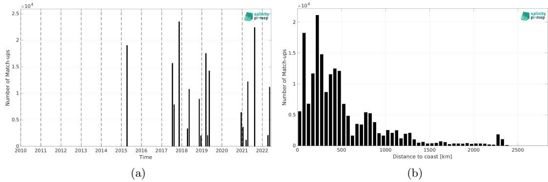
Figure 1: Number of match-ups between TSG (CSIC-UTM) and SMAP SSS L2 v5 (RSS) SSS as a function of time (a) and as function of the distance to coast (b) over the Tropical Atlantic Ocean Pi-MEP region and for the full satellite product period.
