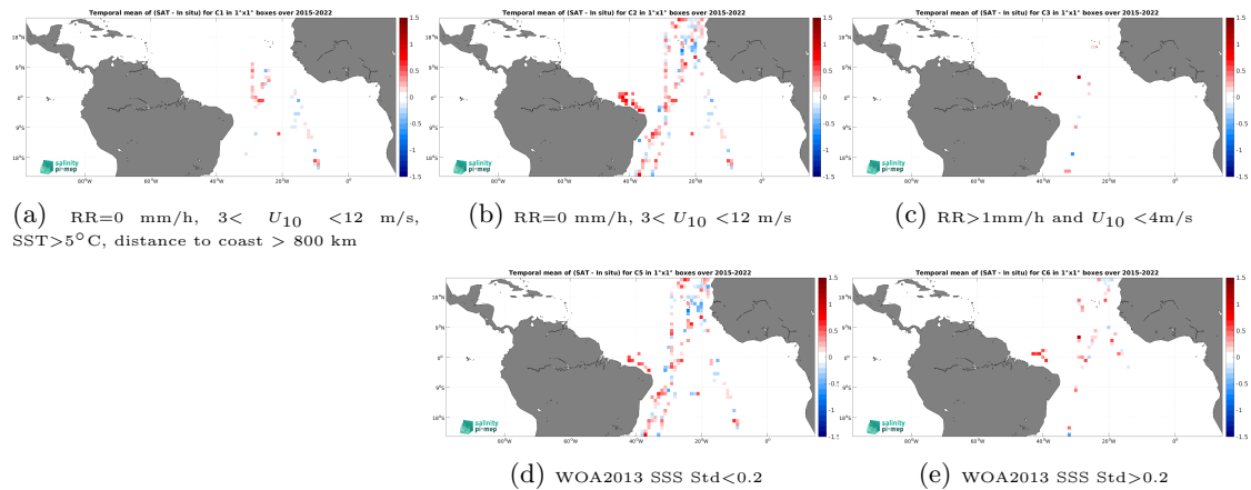
Figure 12: Temporal mean gridded over spatial boxes of size 1^\circ \times 1^\circ of \Delta\text{SSS} (SMAP SSS L2 v5 (RSS) - TSG (CSIC-UTM)) for 5 different subdatasets corresponding to:RR=0 mm/h, 3 < U_{10} < 12 m/s, SST >5^\circ\text{C} , distance to coast > 800 km (a), RR=0 mm/h, 3 < U_{10} < 12 m/s (b), RR >1 mm/h and U_{10} < 4 m/s (c), WOA2013 SSS Std <0.2 (d), WOA2013 SSS Std >0.2 (e).
