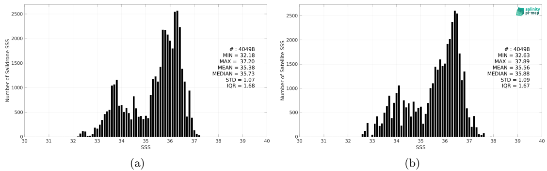
Figure 2: Histograms of SSS from Saildrone (a) and SMAP SSS L2 v5 (RSS) (b) considering all match-up pairs per bins of 0.1 over the Tropical Atlantic Ocean Pi-MEP region and for the full satellite product period.
