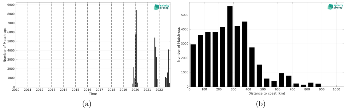
Figure 1: Number of match-ups between Saildrone and SMAP SSS L2 v5 (RSS) SSS as a function of time (a) and as function of the distance to coast (b) over the Tropical Atlantic Ocean Pi-MEP region and for the full satellite product period.
