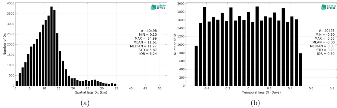
Figure 5: Histograms of the spatial (a) and temporal (b) lags between the location/time of the Smaildrone measurement and the date of the corresponding SMAP SSS L2 v5 (RSS) SSS pixel.
