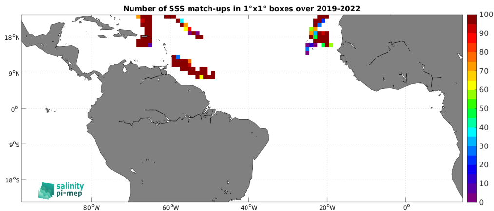
Figure 4: Number of SSS match-ups between Saildrone SSS and the SMAP SSS L2 v5 (RSS) SSS product for the Tropical Atlantic Ocean Pi-MEP region over 1^\circ \times 1^\circ boxes and for the full satellite product period.
