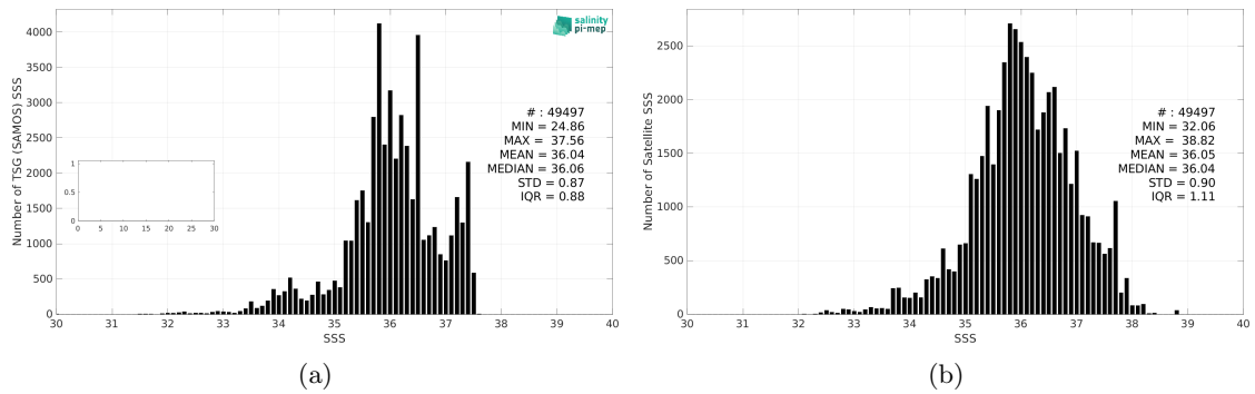
Figure 3: Histograms of SSS from TSG (SAMOS) (a) and SMAP SSS L2 v5.3 (RSS) (b) considering all match-up pairs per bins of 0.1 over the Tropical Atlantic Ocean Pi-MEP region and for the full satellite product period.
