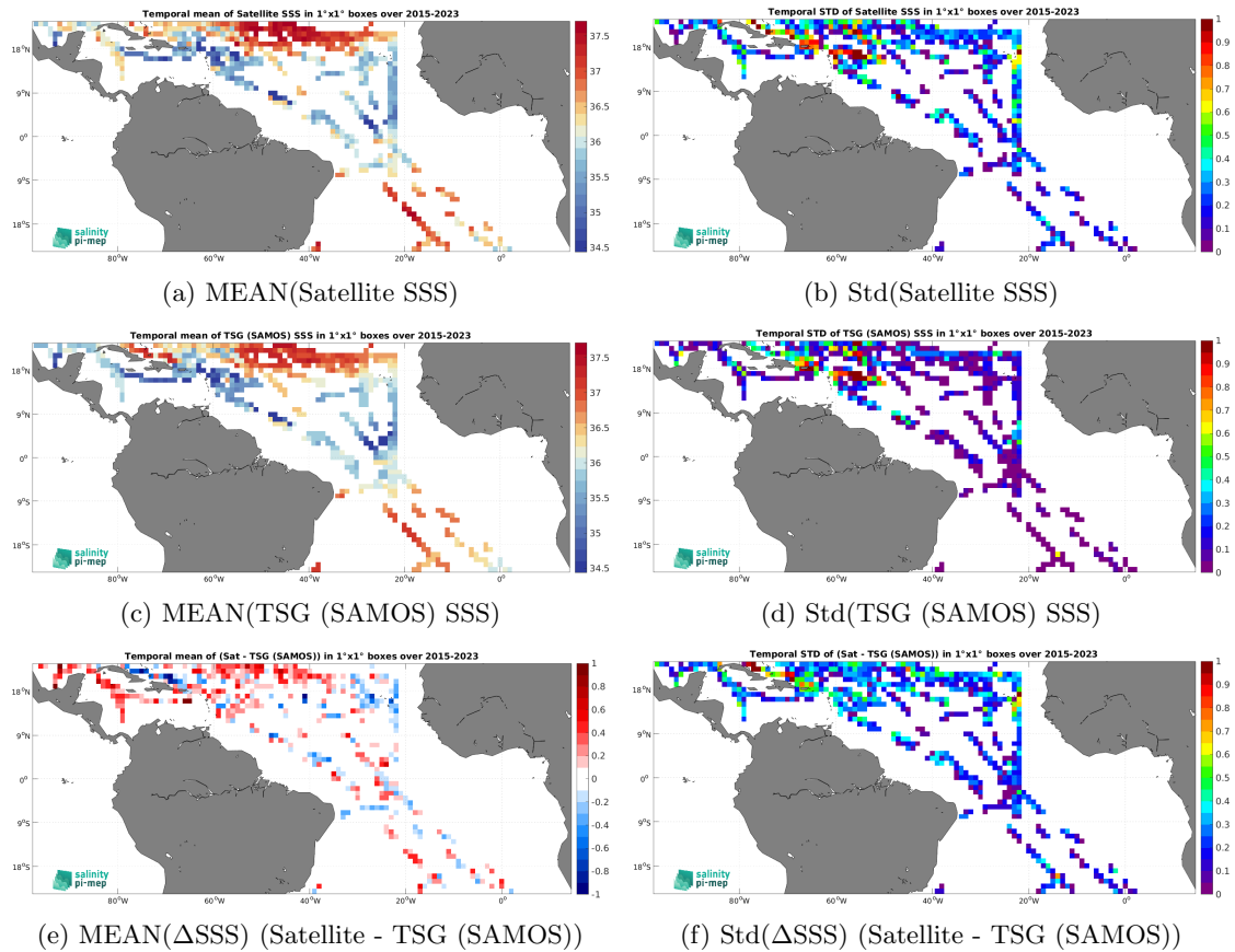
Figure 7: Temporal mean (left) and Std (right) of SSS from SMAP SSS L2 v5.3 (RSS) (top), TSG (SAMOS) (middle), and of \Delta SSS (Satellite - TSG (SAMOS)). Only match-up pairs are used to generate these maps.
