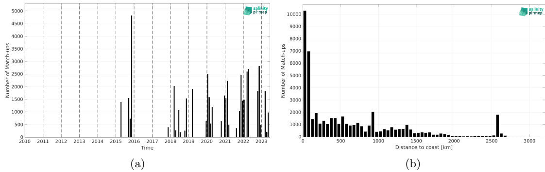
Figure 2: Number of match-ups between TSG (SAMOS) and SMAP SSS L2 v5.3 (RSS) SSS as a function of time (a) and as function of the distance to coast (b) over the Tropical Atlantic Ocean Pi-MEP region and for the full satellite product period.
