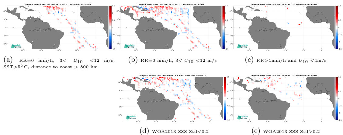
Figure 14: Temporal mean gridded over spatial boxes of size 1^\circ \times 1^\circ of \Delta SSS (SMAP SSS L2 v5.3 (RSS) - TSG (SAMOS)) for 5 different subdatasets corresponding to:RR=0 mm/h, 3 < U_{10} < 12 m/s, SST>5°C, distance to coast > 800 km (a), RR=0 mm/h, 3 < U_{10} < 12 m/s (b), RR>1mm/h and U_{10} < 4 m/s (c), WOA2013 SSS Std<0.2 (d), WOA2013 SSS Std>0.2 (e).
