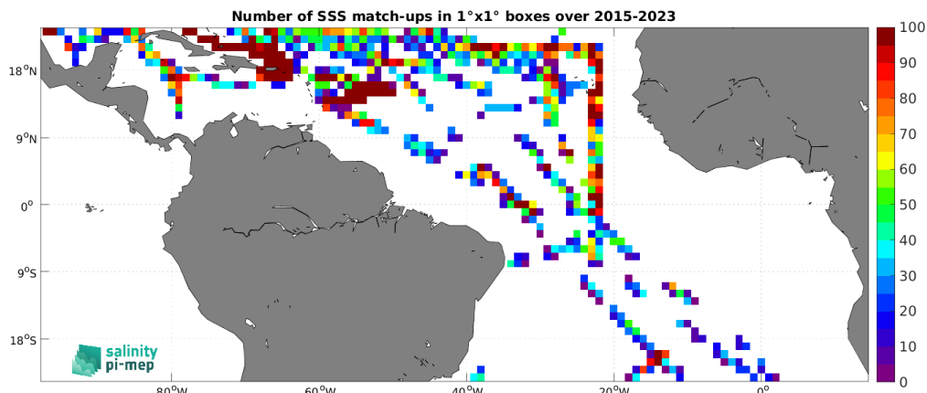
Figure 5: Number of SSS match-ups between TSG (SAMOS) SSS and the SMAP SSS L2 v5.3 (RSS) SSS product for the Tropical Atlantic Ocean Pi-MEP region over 1^\circ \times 1^\circ boxes and for the full satellite product period.
