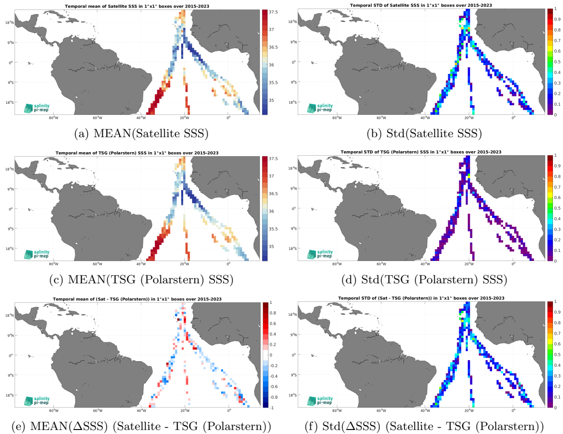
Figure 7: Temporal mean (left) and Std (right) of SSS from SMAP SSS L2 v5.3 (RSS) (top), TSG (Polarstern) (middle), and of \Delta SSS (Satellite - TSG (Polarstern)). Only match-up pairs are used to generate these maps.
