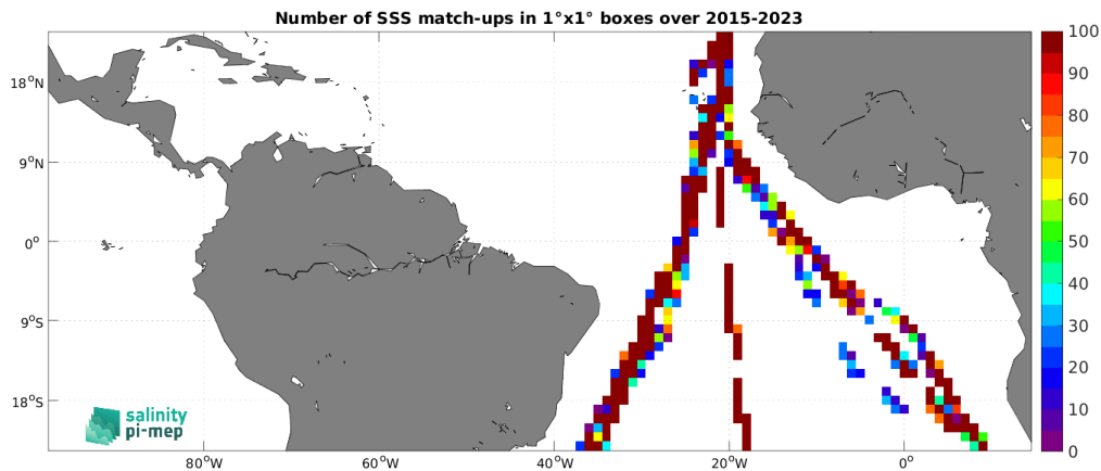
Figure 5: Number of SSS match-ups between TSG (Polarstern) SSS and the SMAP SSS L2 v5.3 (RSS) SSS product for the Tropical Atlantic Ocean Pi-MEP region over 1^\circ \times 1^\circ boxes and for the full satellite product period.
