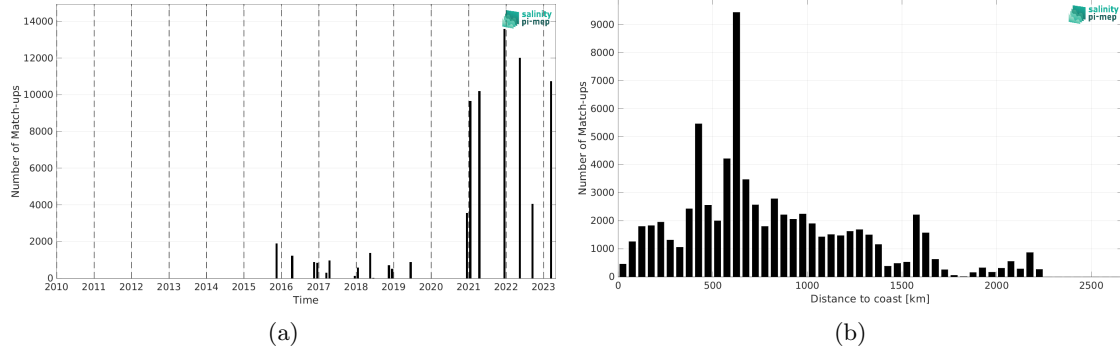
Figure 2: Number of match-ups between TSG (Polarstern) and SMAP SSS L2 v5.3 (RSS) SSS as a function of time (a) and as function of the distance to coast (b) over the Tropical Atlantic Ocean Pi-MEP region and for the full satellite product period.
