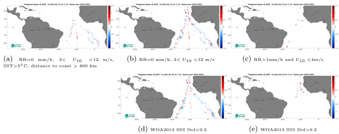
Figure 14: Temporal mean gridded over spatial boxes of size 1^\circ \times 1^\circ of \Delta\text{SSS} (SMAP SSS L2 v5.3 (RSS) - TSG (Polarstern)) for 5 different subdatasets corresponding to:RR=0 mm/h, 3 < U_{10} < 12 m/s, SST >5^\circ\text{C} , distance to coast > 800 km (a), RR=0 mm/h, 3 < U_{10} < 12 m/s (b), RR >1 mm/h and U_{10} < 4 m/s (c), WOA2013 SSS Std <0.2 (d), WOA2013 SSS Std >0.2 (e).
