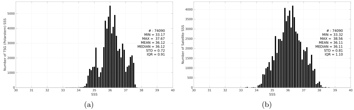
Figure 3: Histograms of SSS from TSG (Polarstern) (a) and SMAP SSS L2 v5.3 (RSS) (b) considering all match-up pairs per bins of 0.1 over the Tropical Atlantic Ocean Pi-MEP region and for the full satellite product period.
