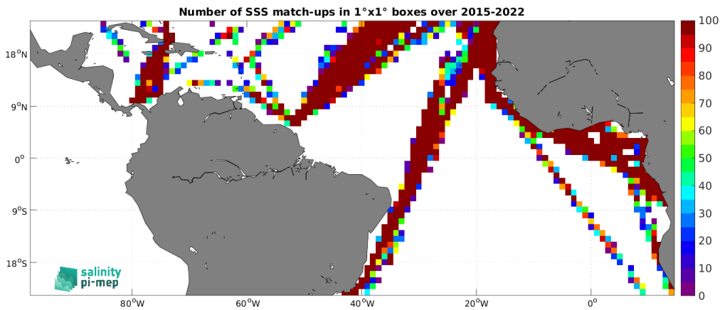
Figure 5: Number of SSS match-ups between TSG (LEGOS-DM) SSS and the SMAP SSS L2 v5.3 (RSS) SSS product for the Tropical Atlantic Ocean Pi-MEP region over 1^\circ \times 1^\circ boxes and for the full satellite product period.
