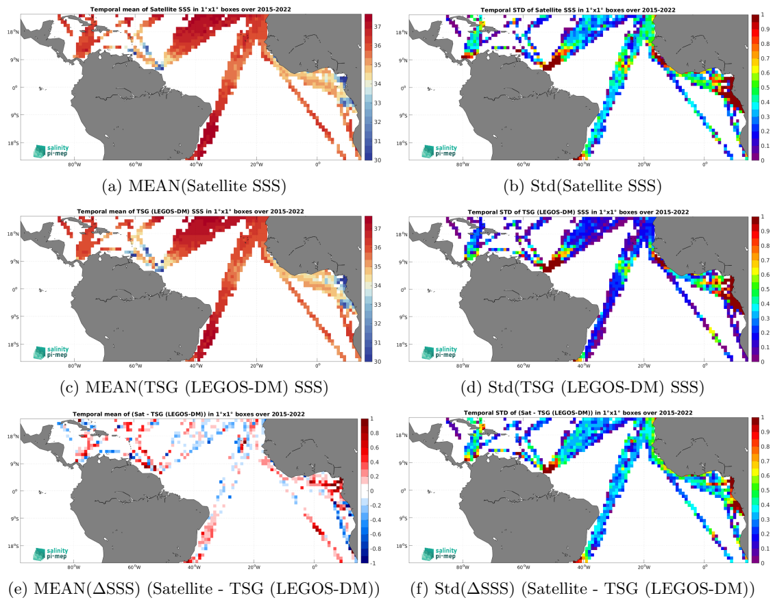
Figure 7: Temporal mean (left) and Std (right) of SSS from SMAP SSS L2 v5.3 (RSS) (top), TSG (LEGOS-DM) (middle), and of \Delta SSS (Satellite - TSG (LEGOS-DM)). Only match-up pairs are used to generate these maps.
