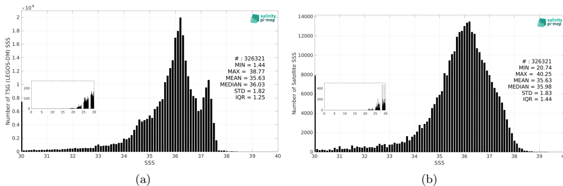
Figure 3: Histograms of SSS from TSG (LEGOS-DM) (a) and SMAP SSS L2 v5.3 (RSS) (b) considering all match-up pairs per bins of 0.1 over the Tropical Atlantic Ocean Pi-MEP region and for the full satellite product period.
