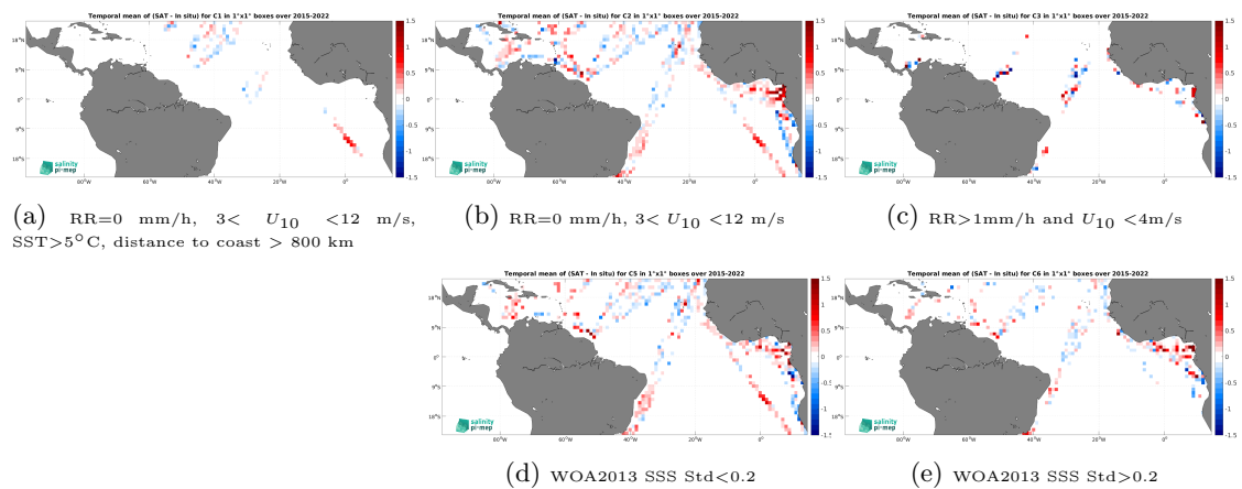
Figure 14: Temporal mean gridded over spatial boxes of size 1^\circ \times 1^\circ of \Delta\text{SSS} (SMAP SSS L2 v5.3 (RSS) - TSG (LEGOS-DM)) for 5 different subdatasets corresponding to:RR=0 mm/h, 3 < U_{10} < 12 m/s, SST >5^\circ\text{C} , distance to coast > 800 km (a), RR=0 mm/h, 3 < U_{10} < 12 m/s (b), RR >1 mm/h and U_{10} < 4 m/s (c), WOA2013 SSS Std <0.2 (d), WOA2013 SSS Std >0.2 (e).
