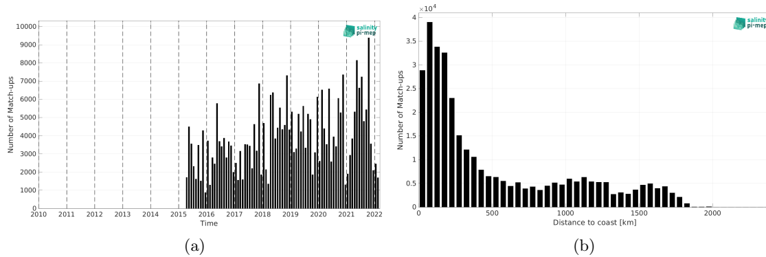
Figure 2: Number of match-ups between TSG (LEGOS-DM) and SMAP SSS L2 v5.3 (RSS) SSS as a function of time (a) and as function of the distance to coast (b) over the Tropical Atlantic Ocean Pi-MEP region and for the full satellite product period.
