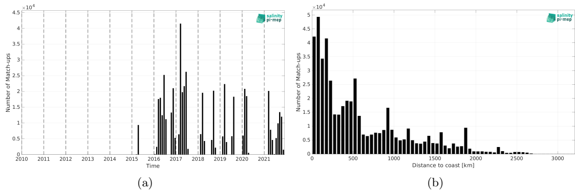
Figure 2: Number of match-ups between TSG (GOSUD-Research-vessel) and SMAP SSS L2 v5.3 (RSS) SSS as a function of time (a) and as function of the distance to coast (b) over the Tropical Atlantic Ocean Pi-MEP region and for the full satellite product period.
