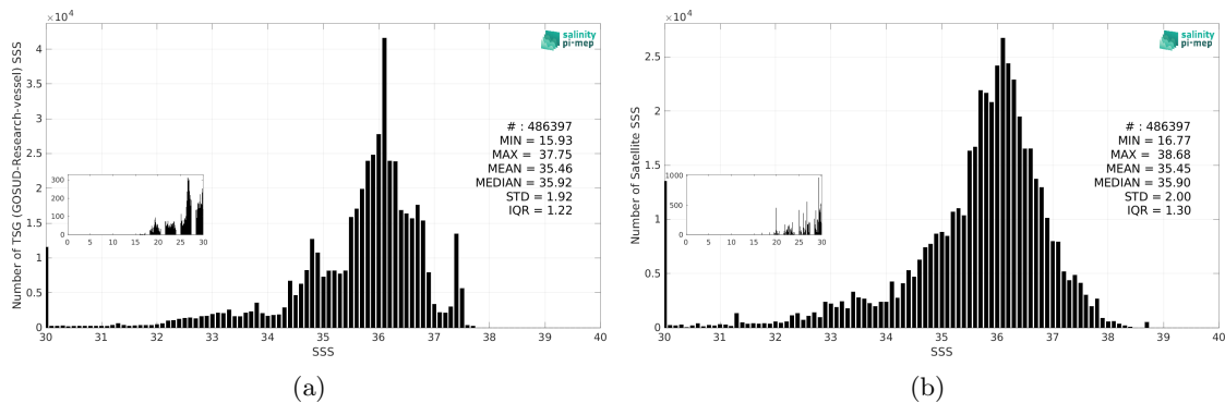
Figure 3: Histograms of SSS from TSG (GOSUD-Research-vessel) (a) and SMAP SSS L2 v5.3 (RSS) (b) considering all match-up pairs per bins of 0.1 over the Tropical Atlantic Ocean Pi-MEP region and for the full satellite product period.
