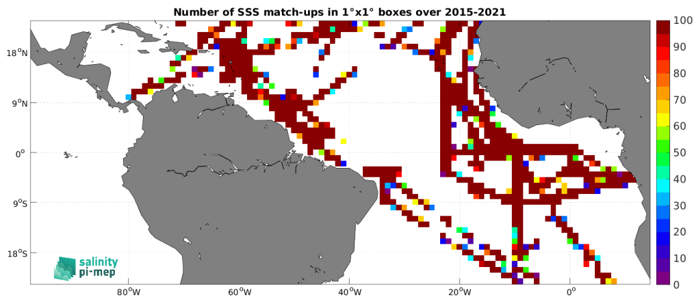
Figure 5: Number of SSS match-ups between TSG (GOSUD-Research-vessel) SSS and the SMAP SSS L2 v5.3 (RSS) SSS product for the Tropical Atlantic Ocean Pi-MEP region over 1°x1° boxes and for the full satellite product period.
