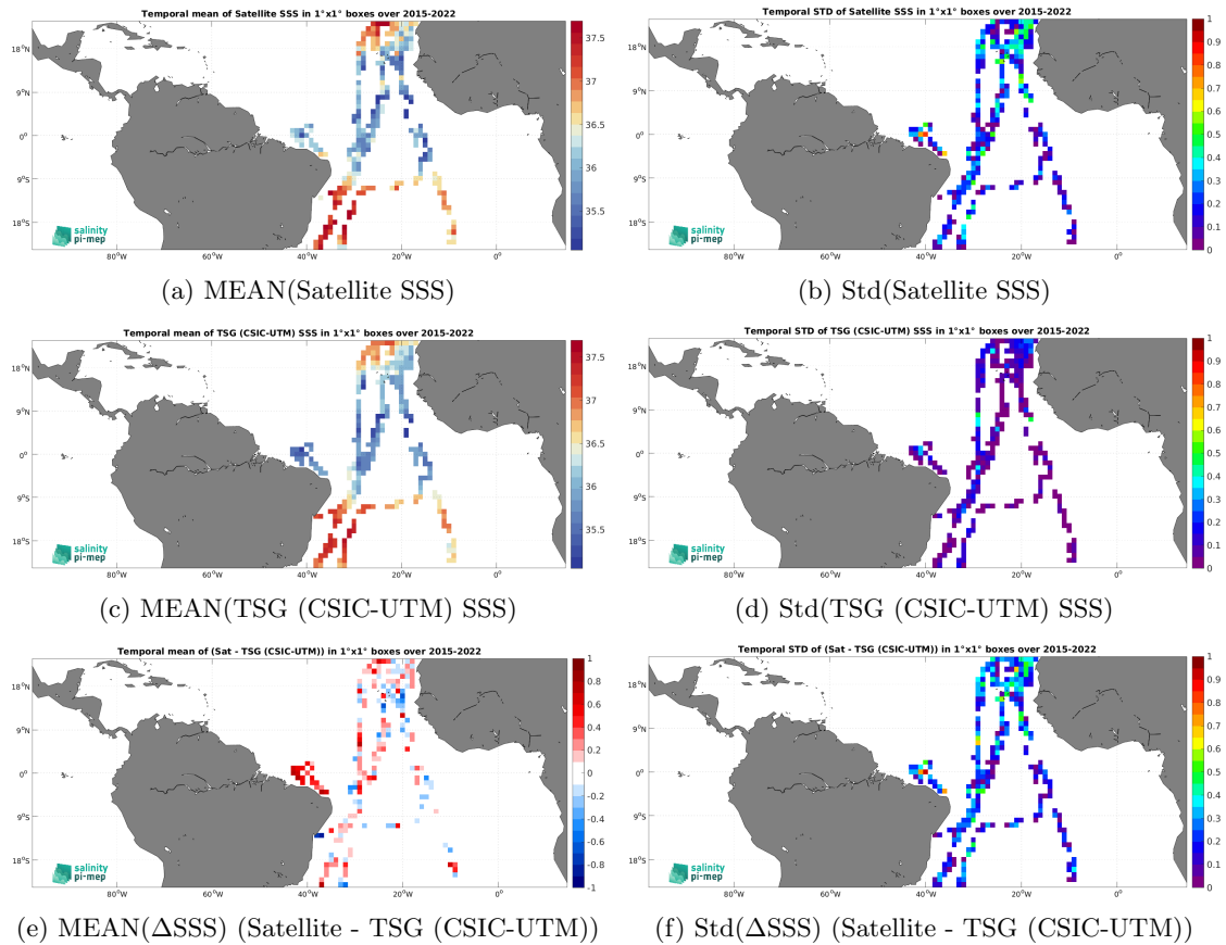
Figure 7: Temporal mean (left) and Std (right) of SSS from SMAP SSS L2 v5.3 (RSS) (top), TSG (CSIC-UTM) (middle), and of \Delta SSS (Satellite - TSG (CSIC-UTM)). Only match-up pairs are used to generate these maps.
