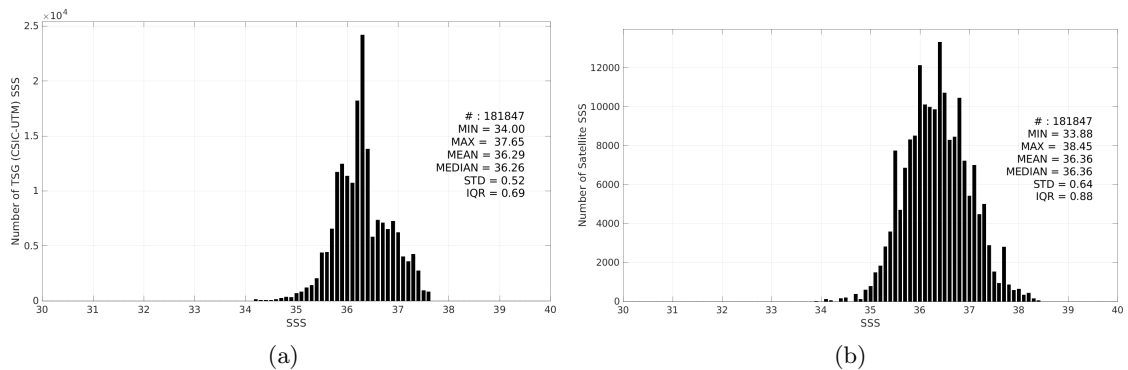
Figure 3: Histograms of SSS from TSG (CSIC-UTM) (a) and SMAP SSS L2 v5.3 (RSS) (b) considering all match-up pairs per bins of 0.1 over the Tropical Atlantic Ocean Pi-MEP region and for the full satellite product period.
