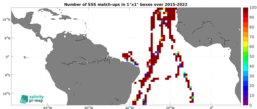
Figure 5: Number of SSS match-ups between TSG (CSIC-UTM) SSS and the SMAP SSS L2 v5.3 (RSS) SSS product for the Tropical Atlantic Ocean Pi-MEP region over 1^\circ \times 1^\circ boxes and for the full satellite product period.
