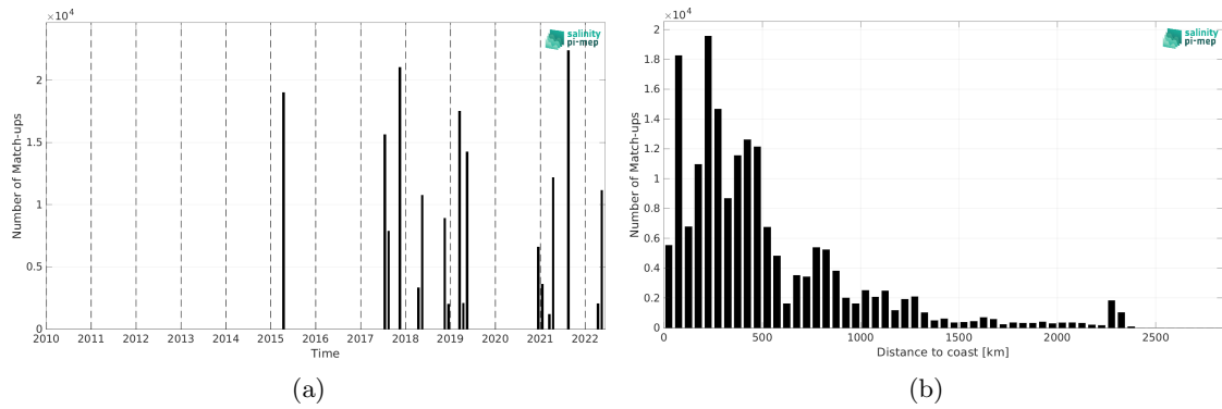
Figure 2: Number of match-ups between TSG (CSIC-UTM) and SMAP SSS L2 v5.3 (RSS) SSS as a function of time (a) and as function of the distance to coast (b) over the Tropical Atlantic Ocean Pi-MEP region and for the full satellite product period.
