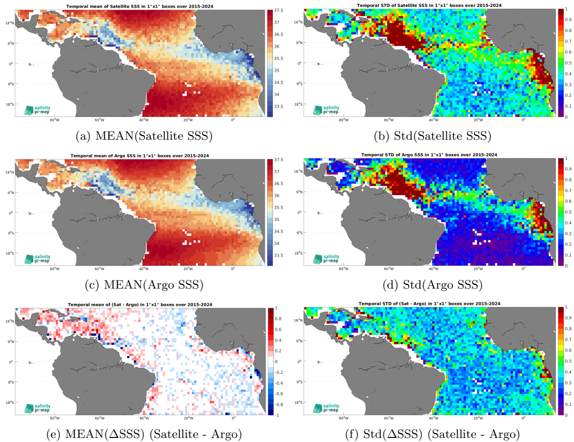
Figure 7: Temporal mean (left) and Std (right) of SSS from SMAP SSS L2 v5.3 (RSS) (top), Argo (middle), and of \Delta SSS (Satellite - Argo). Only match-up pairs are used to generate these maps.
