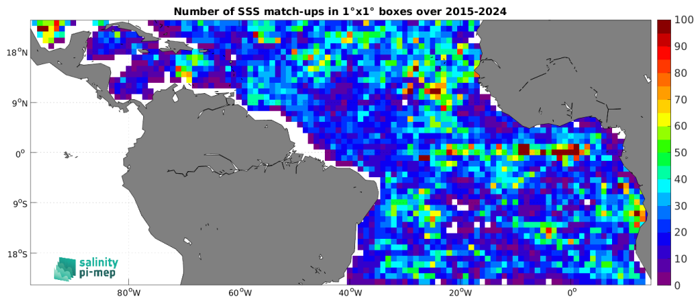
Figure 5: Number of SSS match-ups between Argo SSS and the SMAP SSS L2 v5.3 (RSS) SSS product for the Tropical Atlantic Ocean Pi-MEP region over 1^\circ \times 1^\circ boxes and for the full satellite product period.
