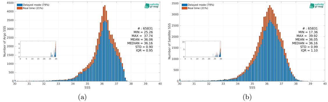
Figure 3: Histograms of SSS from Argo (a) and SMAP SSS L2 v5.3 (RSS) (b) considering all match-up pairs per bins of 0.1 over the Tropical Atlantic Ocean Pi-MEP region and for the full satellite product period.
