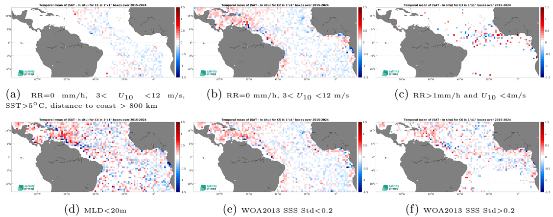
Figure 14: Temporal mean gridded over spatial boxes of size 1^\circ \times 1^\circ of \Delta SSS (SMAP SSS L2 v5.3 (RSS) - Argo) for 6 different subdatasets corresponding to:RR=0 mm/h, 3 < U_{10} < 12 m/s, SST >5^\circ\text{C} , distance to coast > 800 km (a), RR=0 mm/h, 3 < U_{10} < 12 m/s (b), RR >1 mm/h and U_{10} < 4 m/s (c),MLD <20 m (d),WOA2013 SSS Std <0.2 (e),WOA2013 SSS Std >0.2 (f).
