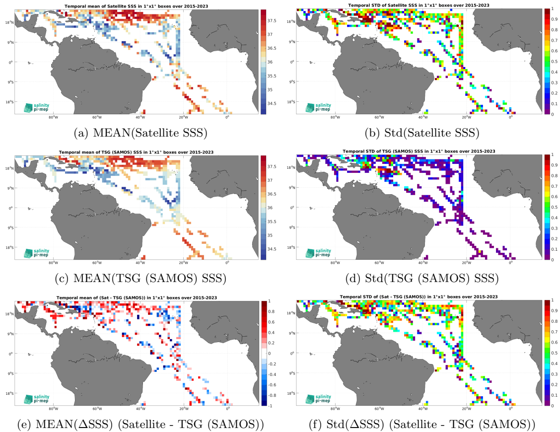
Figure 7: Temporal mean (left) and Std (right) of SSS from SMAP SSS L2 v5.3 - 40 km (RSS) (top), TSG (SAMOS) (middle), and of \Delta SSS (Satellite - TSG (SAMOS)). Only match-up pairs are used to generate these maps.
