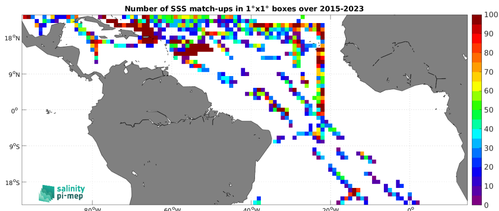
Figure 5: Number of SSS match-ups between TSG (SAMOS) SSS and the SMAP SSS L2 v5.3 - 40 km (RSS) SSS product for the Tropical Atlantic Ocean Pi-MEP region over 1^\circ \times 1^\circ boxes and for the full satellite product period.
