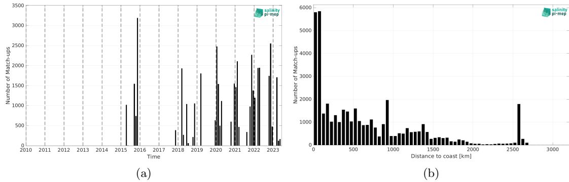
Figure 2: Number of match-ups between TSG (SAMOS) and SMAP SSS L2 v5.3 - 40 km (RSS) SSS as a function of time (a) and as function of the distance to coast (b) over the Tropical Atlantic Ocean Pi-MEP region and for the full satellite product period.
