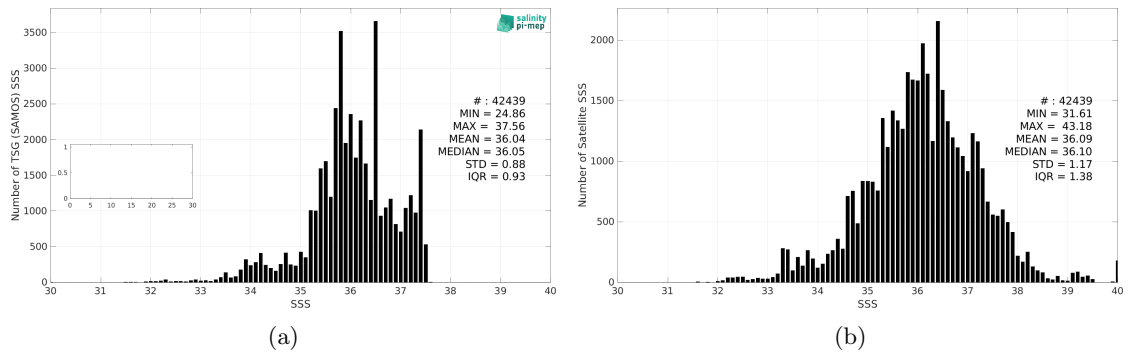
Figure 3: Histograms of SSS from TSG (SAMOS) (a) and SMAP SSS L2 v5.3 - 40 km (RSS) (b) considering all match-up pairs per bins of 0.1 over the Tropical Atlantic Ocean Pi-MEP region and for the full satellite product period.
