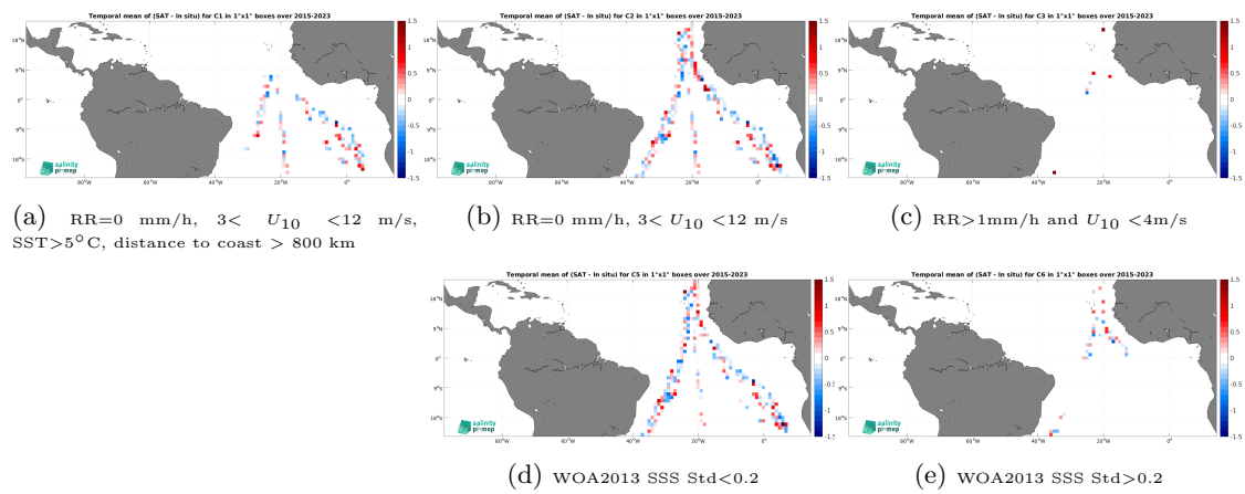
Figure 14: Temporal mean gridded over spatial boxes of size 1^\circ \times 1^\circ of \Delta\text{SSS} (SMAP SSS L2 v5.3 - 40 km (RSS) - TSG (Polarstern)) for 5 different subdatasets corresponding to: RR=0 mm/h, 3 < U_{10} < 12 m/s, SST > 5°C, distance to coast > 800 km (a), RR=0 mm/h, 3 < U_{10} < 12 m/s (b), RR > 1 mm/h and U_{10} < 4 m/s (c), WOA2013 SSS Std < 0.2 (d), WOA2013 SSS Std > 0.2 (e).
