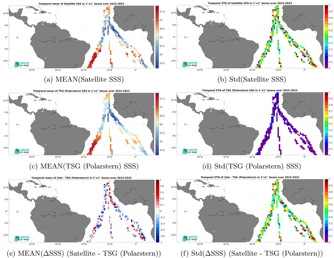
Figure 7: Temporal mean (left) and Std (right) of SSS from SMAP SSS L2 v5.3 - 40 km (RSS) (top), TSG (Polarstern) (middle), and of \Delta SSS (Satellite - TSG (Polarstern)). Only match-up pairs are used to generate these maps.
