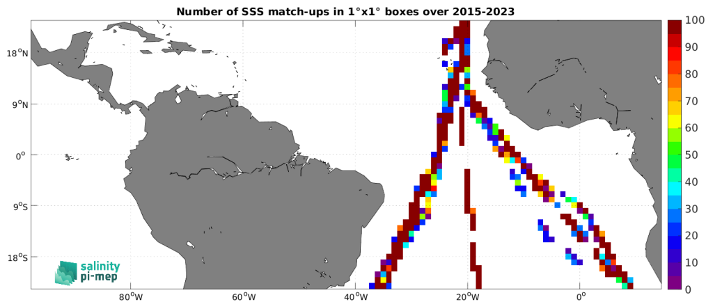
Figure 5: Number of SSS match-ups between TSG (Polarstern) SSS and the SMAP SSS L2 v5.3 - 40 km (RSS) SSS product for the Tropical Atlantic Ocean Pi-MEP region over 1^\circ \times 1^\circ boxes and for the full satellite product period.
