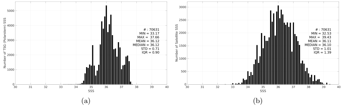
Figure 3: Histograms of SSS from TSG (Polarstern) (a) and SMAP SSS L2 v5.3 - 40 km (RSS) (b) considering all match-up pairs per bins of 0.1 over the Tropical Atlantic Ocean Pi-MEP region and for the full satellite product period.
