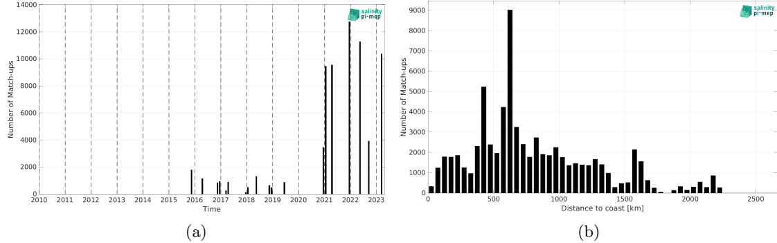
Figure 2: Number of match-ups between TSG (Polarstern) and SMAP SSS L2 v5.3 - 40 km (RSS) SSS as a function of time (a) and as function of the distance to coast (b) over the Tropical Atlantic Ocean Pi-MEP region and for the full satellite product period.
