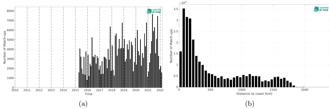
Figure 2: Number of match-ups between TSG (LEGOS-DM) and SMAP SSS L2 v5.3 - 40 km (RSS) SSS as a function of time (a) and as function of the distance to coast (b) over the Tropical Atlantic Ocean Pi-MEP region and for the full satellite product period.
