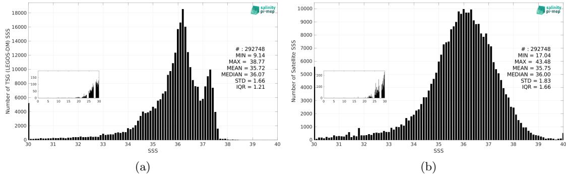
Figure 3: Histograms of SSS from TSG (LEGOS-DM) (a) and SMAP SSS L2 v5.3 - 40 km (RSS) (b) considering all match-up pairs per bins of 0.1 over the Tropical Atlantic Ocean Pi-MEP region and for the full satellite product period.
