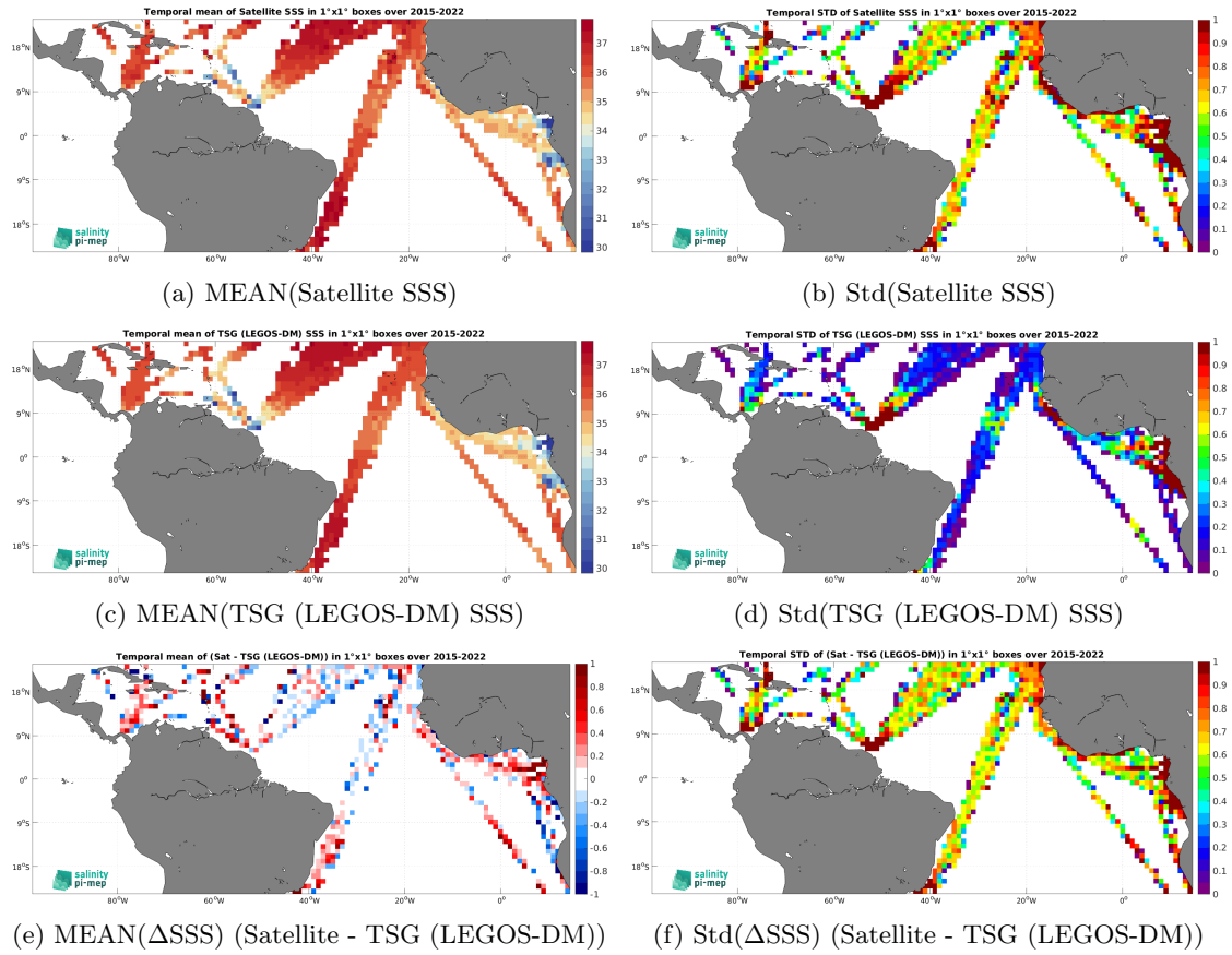
Figure 7: Temporal mean (left) and Std (right) of SSS from SMAP SSS L2 v5.3 - 40 km (RSS) (top), TSG (LEGOS-DM) (middle), and of \Delta SSS (Satellite - TSG (LEGOS-DM)). Only match-up pairs are used to generate these maps.
