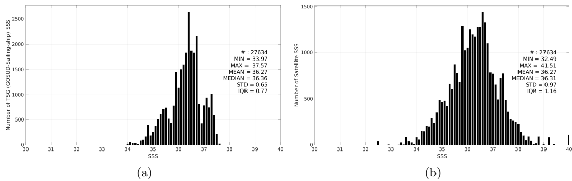
Figure 3: Histograms of SSS from TSG (GOSUD-Sailing-ship) (a) and SMAP SSS L2 v5.3 - 40 km (RSS) (b) considering all match-up pairs per bins of 0.1 over the Tropical Atlantic Ocean Pi-MEP region and for the full satellite product period.
