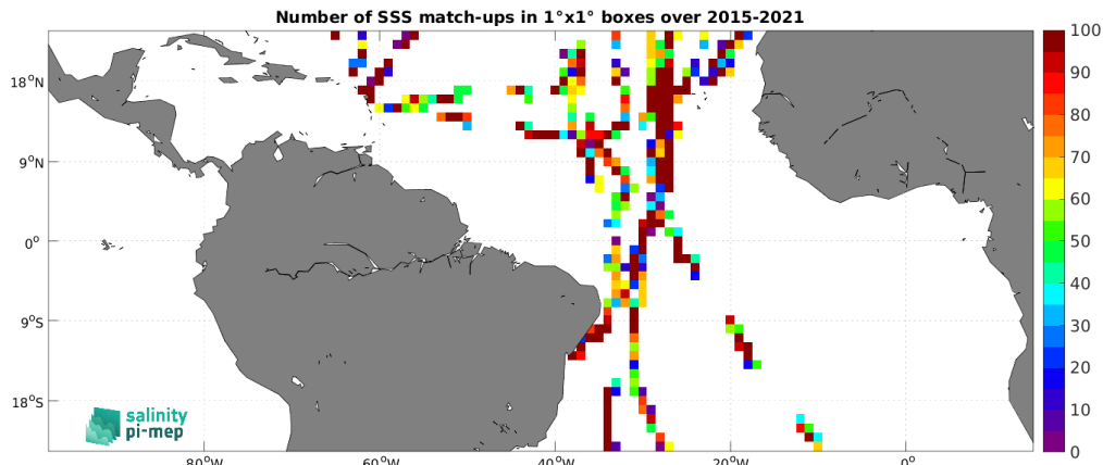
Figure 5: Number of SSS match-ups between TSG (GOSUD-Sailing-ship) SSS and the SMAP SSS L2 v5.3 - 40 km (RSS) SSS product for the Tropical Atlantic Ocean Pi-MEP region over 1^\circ \times 1^\circ boxes and for the full satellite product period.
