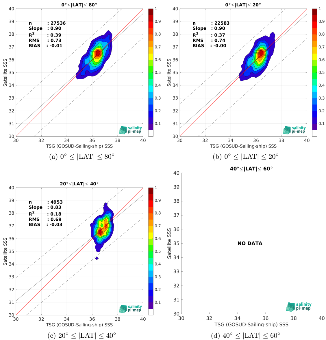
Figure 10: Contour maps of the concentration of SMAP SSS L2 v5.3 - 40 km (RSS) SSS (y-axis) versus TSG (GOSUD-Sailing-ship) SSS (x-axis) at match-up pairs for different latitude bands. For each plot, the red line shows x=y . The black thin and dashed lines indicate a linear fit through the data cloud and the \pm 95\% confidence levels, respectively. The number match-up pairs n , the slope and R^2 coefficient of the linear fit, the root mean square (RMS) and the mean bias between satellite and in situ data are indicated for each latitude band in each plots.
