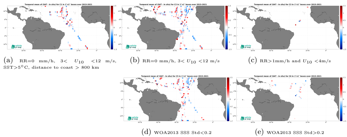
Figure 14: Temporal mean gridded over spatial boxes of size 1^\circ \times 1^\circ of \Delta\text{SSS} (SMAP SSS L2 v5.3 - 40 km (RSS) - TSG (GOSUD-Sailing-ship)) for 5 different subdatasets corresponding to:RR=0 mm/h, 3 < U_{10} < 12 m/s, SST >5^\circ\text{C} , distance to coast > 800 km (a), RR=0 mm/h, 3 < U_{10} < 12 m/s (b), RR >1 mm/h and U_{10} < 4 m/s (c), WOA2013 SSS Std <0.2 (d), WOA2013 SSS Std >0.2 (e).
