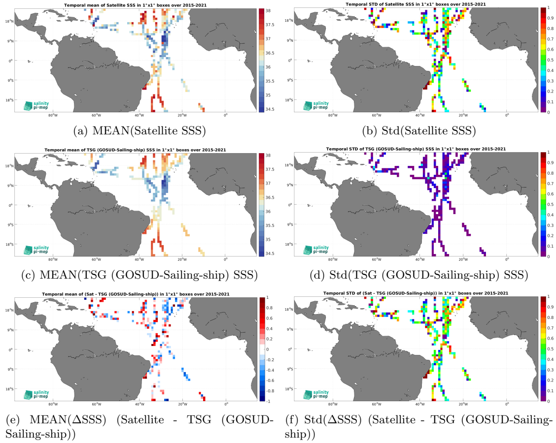
Figure 7: Temporal mean (left) and Std (right) of SSS from SMAP SSS L2 v5.3 - 40 km (RSS) (top), TSG (GOSUD-Sailing-ship) (middle), and of \Delta SSS (Satellite - TSG (GOSUD-Sailing-ship)). Only match-up pairs are used to generate these maps.
