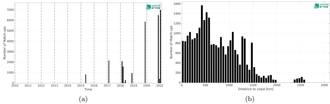
Figure 2: Number of match-ups between TSG (GOSUD-Sailing-ship) and SMAP SSS L2 v5.3 - 40 km (RSS) SSS as a function of time (a) and as function of the distance to coast (b) over the Tropical Atlantic Ocean Pi-MEP region and for the full satellite product period.
