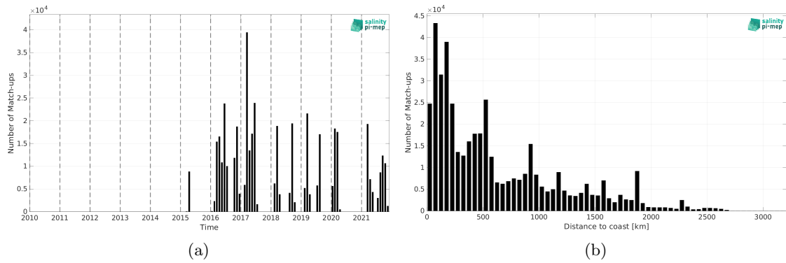
Figure 2: Number of match-ups between TSG (GOSUD-Research-vessel) and SMAP SSS L2 v5.3 - 40 km (RSS) SSS as a function of time (a) and as function of the distance to coast (b) over the Tropical Atlantic Ocean Pi-MEP region and for the full satellite product period.
