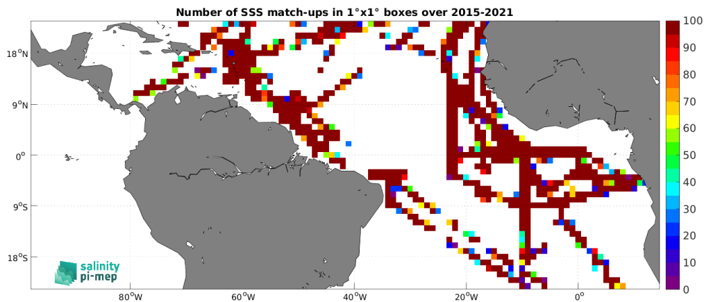
Figure 5: Number of SSS match-ups between TSG (GOSUD-Research-vessel) SSS and the SMAP SSS L2 v5.3 - 40 km (RSS) SSS product for the Tropical Atlantic Ocean Pi-MEP region over 1^\circ \times 1^\circ boxes and for the full satellite product period.
