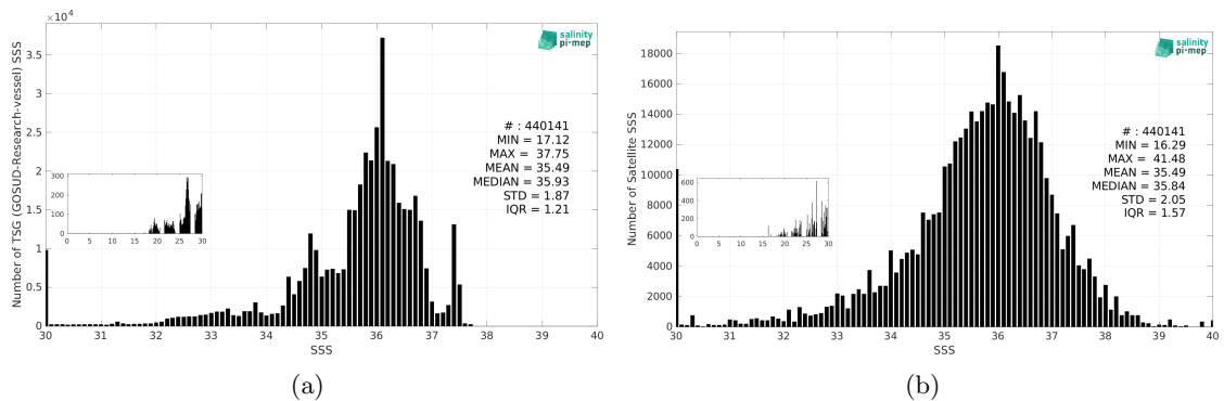
Figure 3: Histograms of SSS from TSG (GOSUD-Research-vessel) (a) and SMAP SSS L2 v5.3 - 40 km (RSS) (b) considering all match-up pairs per bins of 0.1 over the Tropical Atlantic Ocean Pi-MEP region and for the full satellite product period.
