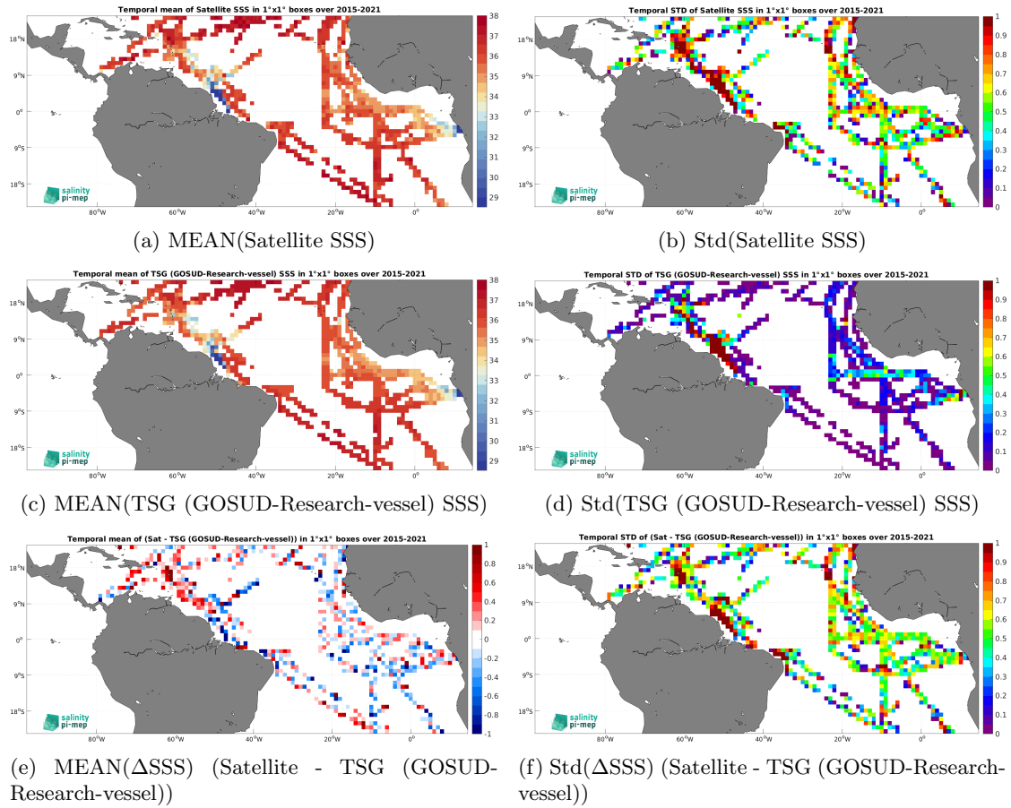
Figure 7: Temporal mean (left) and Std (right) of SSS from SMAP SSS L2 v5.3 - 40 km (RSS) (top), TSG (GOSUD-Research-vessel) (middle), and of \Delta SSS (Satellite - TSG (GOSUD-Research-vessel)). Only match-up pairs are used to generate these maps.
