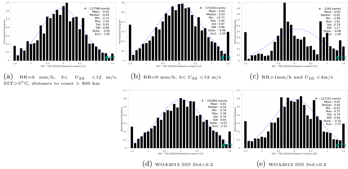
Figure 15: Normalized histogram of \Delta SSS (SMAP SSS L2 v5.3 - 40 km (RSS) - TSG (GOSUD-Research-vessel)) for 5 different subdatasets corresponding to: RR=0 mm/h, 3 < U_{10} < 12 m/s, SST>5°C, distance to coast > 800 km (a), RR=0 mm/h, 3 < U_{10} < 12 m/s (b), RR>1mm/h and U_{10} < 4 m/s (c), WOA2013 SSS Std<0.2 (d), WOA2013 SSS Std>0.2 (e).
