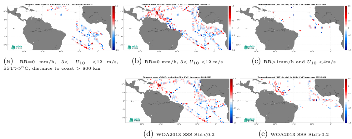
Figure 14: Temporal mean gridded over spatial boxes of size 1^\circ \times 1^\circ of \Delta\text{SSS} (SMAP SSS L2 v5.3 - 40 km (RSS) - TSG (GOSUD-Research-vessel)) for 5 different subdatasets corresponding to:RR=0 mm/h, 3 < U_{10} < 12 m/s, SST>5°C, distance to coast > 800 km (a), RR=0 mm/h, 3 < U_{10} < 12 m/s (b), RR>1mm/h and U_{10} < 4 m/s (c), WOA2013 SSS Std<0.2 (d), WOA2013 SSS Std>0.2 (e).
