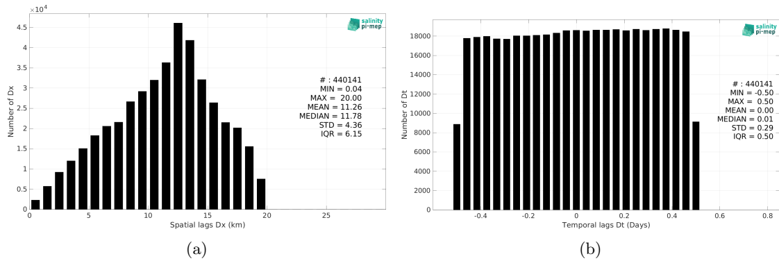
Figure 6: Histograms of the spatial (a) and temporal (b) lags between the location/time of the TSG (GOSUD-Research-vessel) measurement and the date of the corresponding SMAP SSS L2 v5.3 - 40 km (RSS) SSS pixel.
