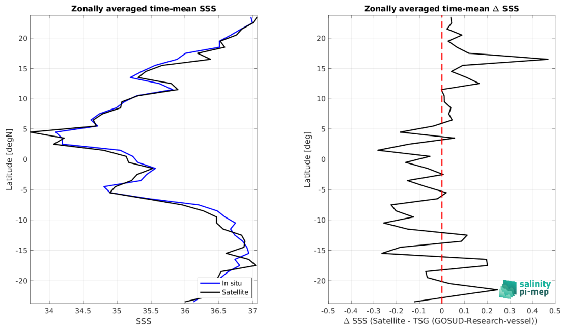
Figure 9: Left panel: Zonal mean SSS from SMAP SSS L2 v5.3 - 40 km (RSS) satellite product (black) and from TSG (GOSUD-Research-vessel) (blue). Right panel: Zonal mean of \Delta SSS (Satellite - TSG (GOSUD-Research-vessel)) for all the collected Pi-MEP match-up pairs estimated over the full satellite product period.
