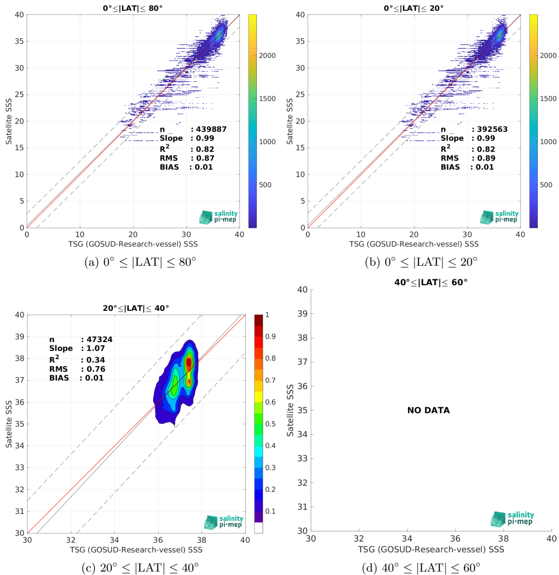
Figure 10: Contour maps of the concentration of SMAP SSS L2 v5.3 - 40 km (RSS) SSS (y-axis) versus TSG (GOSUD-Research-vessel) SSS (x-axis) at match-up pairs for different latitude bands. For each plot, the red line shows x=y . The black thin and dashed lines indicate a linear fit through the data cloud and the \pm 95\% confidence levels, respectively. The number match-up pairs n , the slope and R^2 coefficient of the linear fit, the root mean square (RMS) and the mean bias between satellite and in situ data are indicated for each latitude band in each plots.
