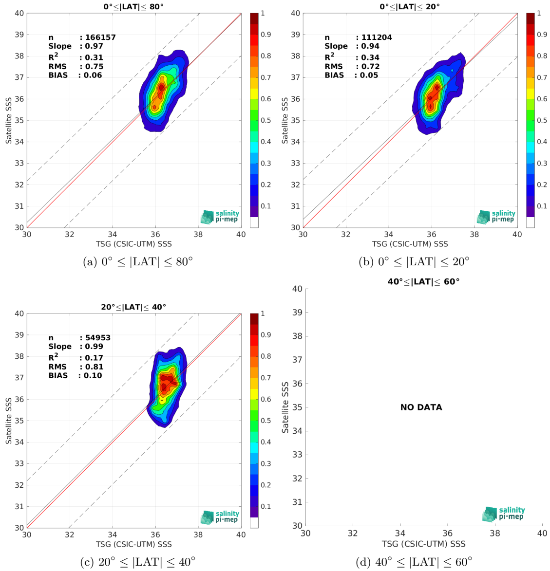
Figure 10: Contour maps of the concentration of SMAP SSS L2 v5.3 - 40 km (RSS) SSS (y-axis) versus TSG (CSIC-UTM) SSS (x-axis) at match-up pairs for different latitude bands. For each plot, the red line shows x=y . The black thin and dashed lines indicate a linear fit through the data cloud and the \pm 95\% confidence levels, respectively. The number match-up pairs n , the slope and R^2 coefficient of the linear fit, the root mean square (RMS) and the mean bias between satellite and in situ data are indicated for each latitude band in each plots.
