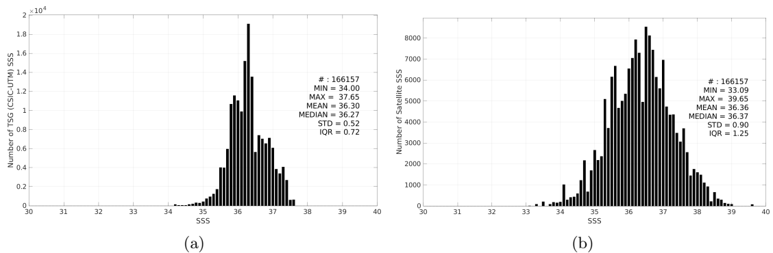
Figure 3: Histograms of SSS from TSG (CSIC-UTM) (a) and SMAP SSS L2 v5.3 - 40 km (RSS) (b) considering all match-up pairs per bins of 0.1 over the Tropical Atlantic Ocean Pi-MEP region and for the full satellite product period.
