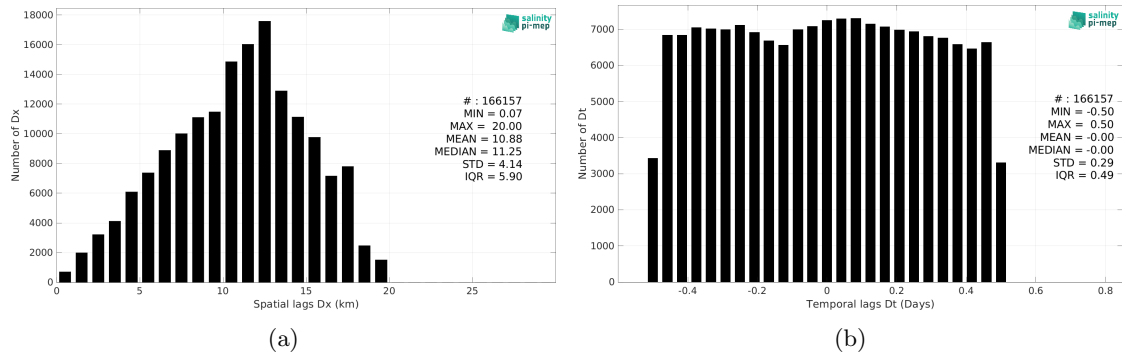
Figure 6: Histograms of the spatial (a) and temporal (b) lags between the location/time of the TSG (CSIC-UTM) measurement and the date of the corresponding SMAP SSS L2 v5.3 - 40 km (RSS) SSS pixel.
