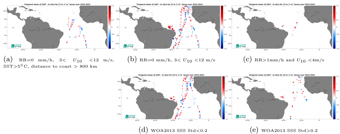
Figure 14: Temporal mean gridded over spatial boxes of size 1^\circ \times 1^\circ of \Delta\text{SSS} (SMAP SSS L2 v5.3 - 40 km (RSS) - TSG (CSIC-UTM)) for 5 different subdatasets corresponding to:RR=0 mm/h, 3 < U_{10} < 12 m/s, SST >5^\circ\text{C} , distance to coast > 800 km (a), RR=0 mm/h, 3 < U_{10} < 12 m/s (b), RR >1 mm/h and U_{10} < 4 m/s (c), WOA2013 SSS Std <0.2 (d), WOA2013 SSS Std >0.2 (e).
