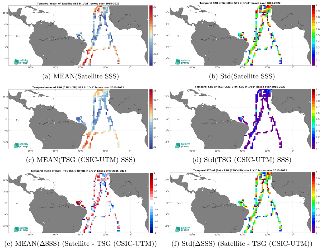
Figure 7: Temporal mean (left) and Std (right) of SSS from SMAP SSS L2 v5.3 - 40 km (RSS) (top), TSG (CSIC-UTM) (middle), and of \Delta SSS (Satellite - TSG (CSIC-UTM)). Only match-up pairs are used to generate these maps.
