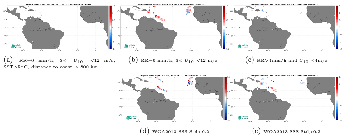
Figure 14: Temporal mean gridded over spatial boxes of size 1^\circ \times 1^\circ of \Delta\text{SSS} (SMAP SSS L2 v5.3 - 40 km (RSS) - Sailability) for 5 different subdatasets corresponding to:RR=0 mm/h, 3 < U_{10} < 12 m/s, SST >5^\circ\text{C} , distance to coast > 800 km (a), RR=0 mm/h, 3 < U_{10} < 12 m/s (b), RR >1 mm/h and U_{10} < 4 m/s (c), WOA2013 SSS Std <0.2 (d), WOA2013 SSS Std >0.2 (e).
