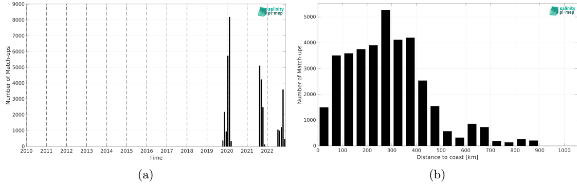
Figure 2: Number of match-ups between Saildrone and SMAP SSS L2 v5.3 - 40 km (RSS) SSS as a function of time (a) and as function of the distance to coast (b) over the Tropical Atlantic Ocean Pi-MEP region and for the full satellite product period.
