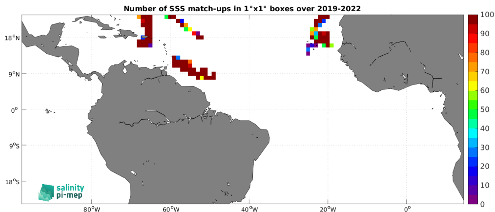
Figure 5: Number of SSS match-ups between Saildrone SSS and the SMAP SSS L2 v5.3 - 40 km (RSS) SSS product for the Tropical Atlantic Ocean Pi-MEP region over 1^\circ \times 1^\circ boxes and for the full satellite product period.
