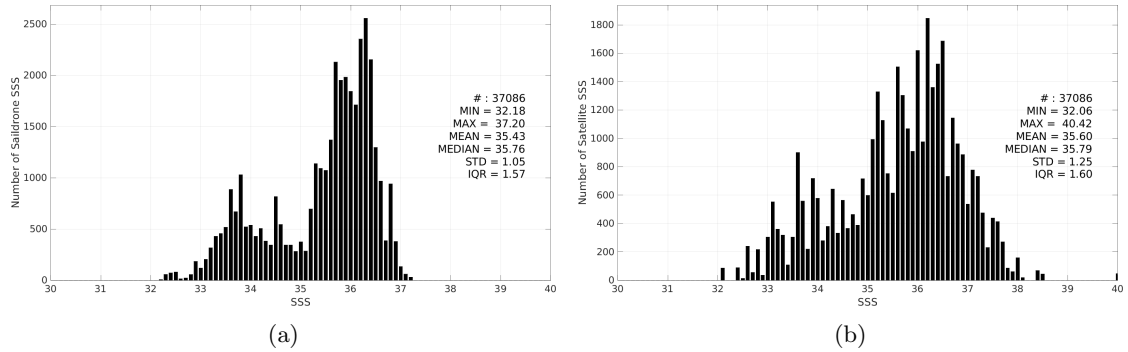
Figure 3: Histograms of SSS from Saildrone (a) and SMAP SSS L2 v5.3 - 40 km (RSS) (b) considering all match-up pairs per bins of 0.1 over the Tropical Atlantic Ocean Pi-MEP region and for the full satellite product period.
