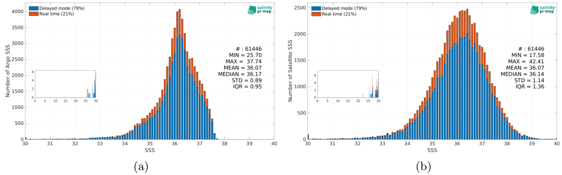
Figure 3: Histograms of SSS from Argo (a) and SMAP SSS L2 v5.3 - 40 km (RSS) (b) considering all match-up pairs per bins of 0.1 over the Tropical Atlantic Ocean Pi-MEP region and for the full satellite product period.
