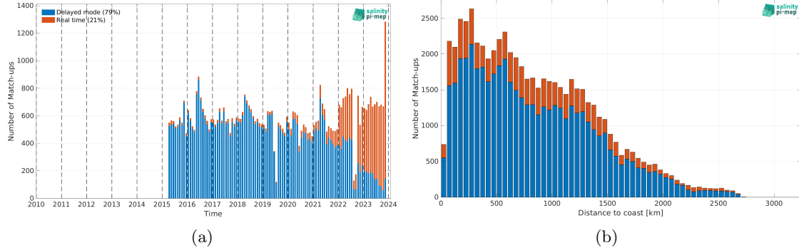
Figure 2: Number of match-ups between Argo and SMAP SSS L2 v5.3 - 40 km (RSS) SSS as a function of time (a) and as function of the distance to coast (b) over the Tropical Atlantic Ocean Pi-MEP region and for the full satellite product period.
