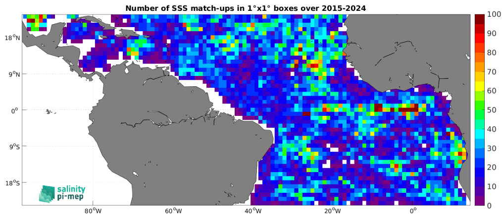
Figure 5: Number of SSS match-ups between Argo SSS and the SMAP SSS L2 v5.3 - 40 km (RSS) SSS product for the Tropical Atlantic Ocean Pi-MEP region over 1^\circ \times 1^\circ boxes and for the full satellite product period.
