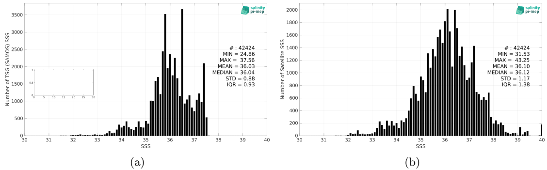
Figure 2: Histograms of SSS from TSG (SAMOS) (a) and SMAP SSS L2 v5 - 40 km (RSS) (b) considering all match-up pairs per bins of 0.1 over the Tropical Atlantic Ocean Pi-MEP region and for the full satellite product period.
