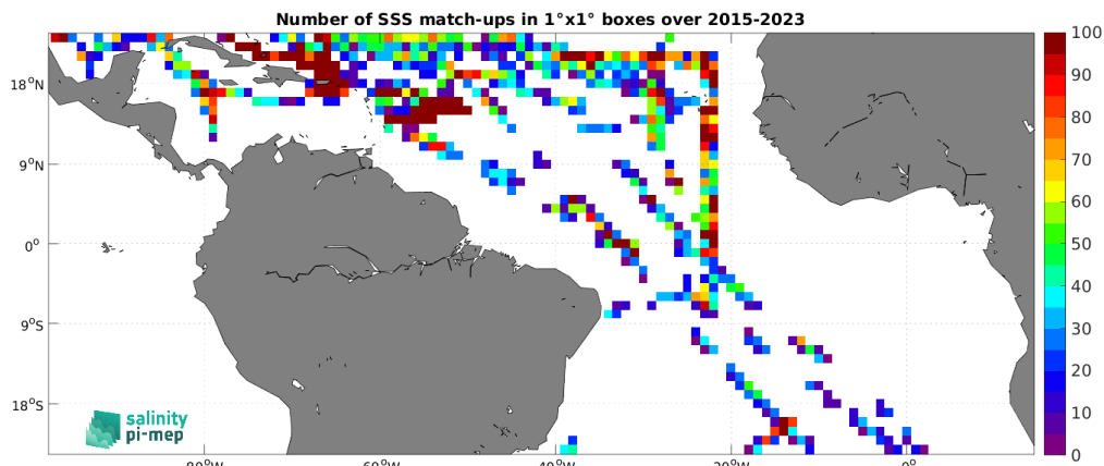
Figure 4: Number of SSS match-ups between TSG (SAMOS) SSS and the SMAP SSS L2 v5 - 40 km (RSS) SSS product for the Tropical Atlantic Ocean Pi-MEP region over 1^\circ \times 1^\circ boxes and for the full satellite product period.
