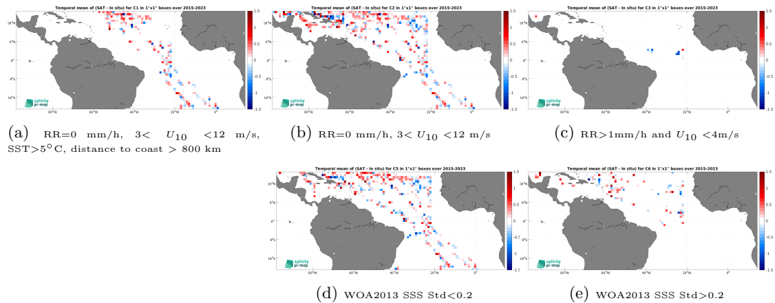
Figure 12: Temporal mean gridded over spatial boxes of size 1^\circ \times 1^\circ of \Delta\text{SSS} (SMAP SSS L2 v5 - 40 km (RSS) - TSG (SAMOS)) for 5 different subdatasets corresponding to:RR=0 mm/h, 3 < U_{10} < 12 m/s, SST >5^\circ\text{C} , distance to coast > 800 km (a), RR=0 mm/h, 3 < U_{10} < 12 m/s (b), RR >1 mm/h and U_{10} < 4 m/s (c), WOA2013 SSS Std <0.2 (d), WOA2013 SSS Std >0.2 (e).
