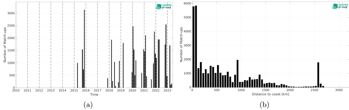
Figure 1: Number of match-ups between TSG (SAMOS) and SMAP SSS L2 v5 - 40 km (RSS) SSS as a function of time (a) and as function of the distance to coast (b) over the Tropical Atlantic Ocean Pi-MEP region and for the full satellite product period.
