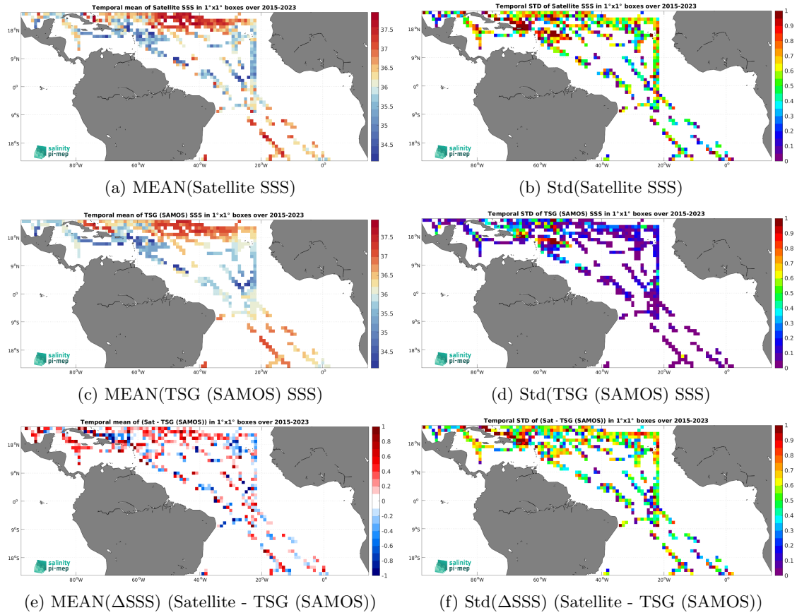
Figure 6: Temporal mean (left) and Std (right) of SSS from SMAP SSS L2 v5 - 40 km (RSS) (top), TSG (SAMOS) (middle), and of \Delta SSS (Satellite - TSG (SAMOS)). Only match-up pairs are used to generate these maps.
