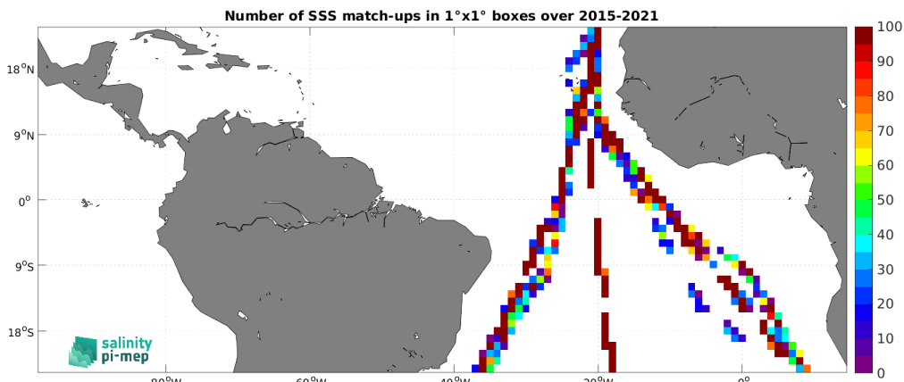
Figure 4: Number of SSS match-ups between TSG (Polarstern) SSS and the SMAP SSS L2 v5 - 40 km (RSS) SSS product for the Tropical Atlantic Ocean Pi-MEP region over 1^\circ \times 1^\circ boxes and for the full satellite product period.
