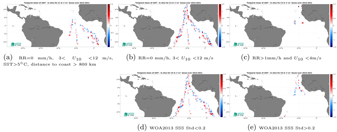
Figure 12: Temporal mean gridded over spatial boxes of size 1^\circ \times 1^\circ of \Delta\text{SSS} (SMAP SSS L2 v5 - 40 km (RSS) - TSG (Polarstern)) for 5 different subdatasets corresponding to:RR=0 mm/h, 3 < U_{10} < 12 m/s, SST >5^\circ\text{C} , distance to coast > 800 km (a), RR=0 mm/h, 3 < U_{10} < 12 m/s (b), RR >1 mm/h and U_{10} < 4 m/s (c), WOA2013 SSS Std <0.2 (d), WOA2013 SSS Std >0.2 (e).
