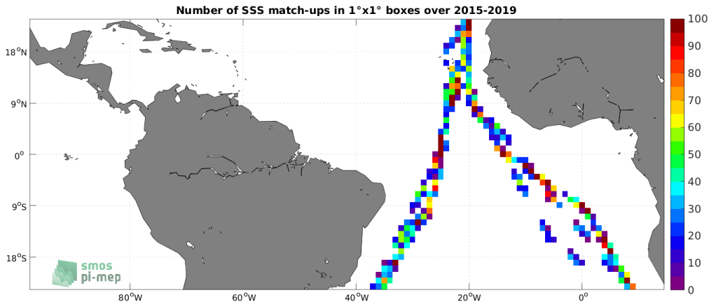
Figure 4: Number of SSS match-ups between TSG (Polarstern) SSS and the SMAP SSS L2 v5 - 40 km (RSS) SSS product for the Tropical Atlantic Ocean Pi-MEP region over 1°x1° boxes and for the full satellite product period.
