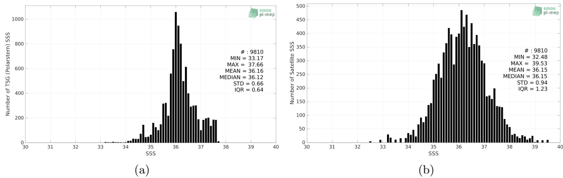
Figure 2: Histograms of SSS from TSG (Polarstern) (a) and SMAP SSS L2 v5 - 40 km (RSS) (b) considering all match-up pairs per bins of 0.1 over the Tropical Atlantic Ocean Pi-MEP region and for the full satellite product period.
