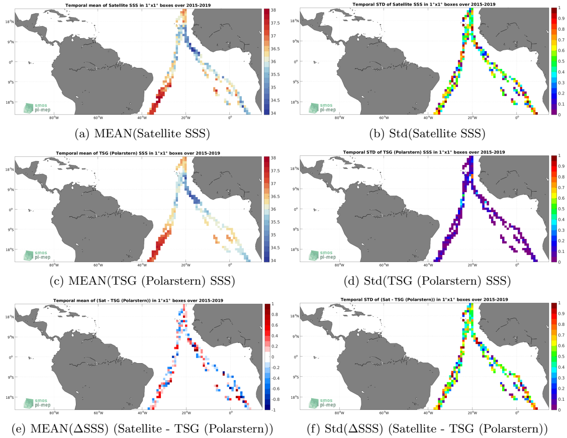
Figure 6: Temporal mean (left) and Std (right) of SSS from SMAP SSS L2 v5 - 40 km (RSS) (top), TSG (Polarstern) (middle), and of \Delta SSS (Satellite - TSG (Polarstern)). Only match-up pairs are used to generate these maps.
