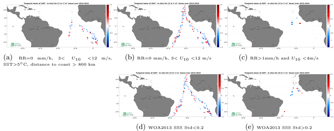
Figure 12: Temporal mean gridded over spatial boxes of size 1^\circ \times 1^\circ of \Delta SSS (SMAP SSS L2 v5 - 40 km (RSS) - TSG (Polarstern)) for 5 different subdatasets corresponding to:RR=0 mm/h, 3 < U_{10} < 12 m/s, SST >5^\circ\text{C} , distance to coast > 800 km (a), RR=0 mm/h, 3 < U_{10} < 12 m/s (b), RR >1 mm/h and U_{10} < 4 m/s (c), WOA2013 SSS Std <0.2 (d), WOA2013 SSS Std >0.2 (e).
