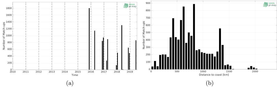
Figure 1: Number of match-ups between TSG (Polarstern) and SMAP SSS L2 v5 - 40 km (RSS) SSS as a function of time (a) and as function of the distance to coast (b) over the Tropical Atlantic Ocean Pi-MEP region and for the full satellite product period.
