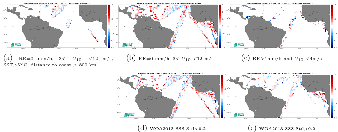
Figure 12: Temporal mean gridded over spatial boxes of size 1^\circ \times 1^\circ of \Delta\text{SSS} (SMAP SSS L2 v5 - 40 km (RSS) - TSG (LEGOS-DM)) for 5 different subdatasets corresponding to:RR=0 mm/h, 3 < U_{10} < 12 m/s, SST >5^\circ\text{C} , distance to coast > 800 km (a), RR=0 mm/h, 3 < U_{10} < 12 m/s (b), RR >1 mm/h and U_{10} < 4 m/s (c), WOA2013 SSS Std <0.2 (d), WOA2013 SSS Std >0.2 (e).
