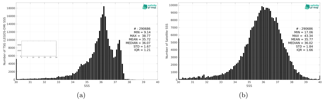
Figure 2: Histograms of SSS from TSG (LEGOS-DM) (a) and SMAP SSS L2 v5 - 40 km (RSS) (b) considering all match-up pairs per bins of 0.1 over the Tropical Atlantic Ocean Pi-MEP region and for the full satellite product period.
