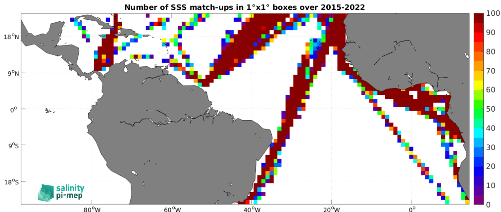
Figure 4: Number of SSS match-ups between TSG (LEGOS-DM) SSS and the SMAP SSS L2 v5 - 40 km (RSS) SSS product for the Tropical Atlantic Ocean Pi-MEP region over 1^\circ \times 1^\circ boxes and for the full satellite product period.
