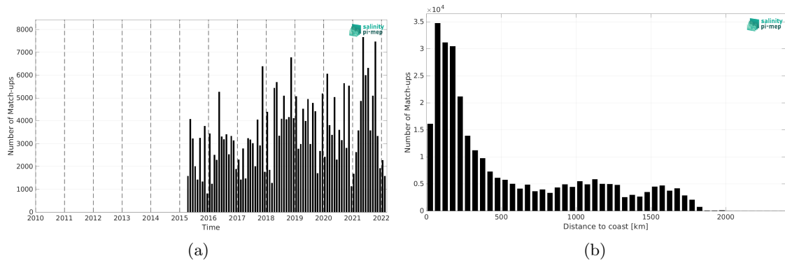
Figure 1: Number of match-ups between TSG (LEGOS-DM) and SMAP SSS L2 v5 - 40 km (RSS) SSS as a function of time (a) and as function of the distance to coast (b) over the Tropical Atlantic Ocean Pi-MEP region and for the full satellite product period.
