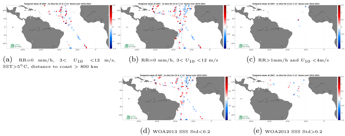
Figure 12: Temporal mean gridded over spatial boxes of size 1^\circ \times 1^\circ of \Delta SSS (SMAP SSS L2 v5 - 40 km (RSS) - TSG (GOSUD-Sailing-ship)) for 5 different subdatasets corresponding to:RR=0 mm/h, 3 < U_{10} < 12 m/s, SST>5°C, distance to coast > 800 km (a), RR=0 mm/h, 3 < U_{10} < 12 m/s (b), RR>1mm/h and U_{10} < 4 m/s (c), WOA2013 SSS Std<0.2 (d), WOA2013 SSS Std>0.2 (e).
