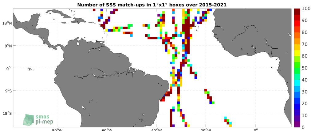
Figure 4: Number of SSS match-ups between TSG (GOSUD-Sailing-ship) SSS and the SMAP SSS L2 v5 - 40 km (RSS) SSS product for the Tropical Atlantic Ocean Pi-MEP region over 1^\circ \times 1^\circ boxes and for the full satellite product period.
