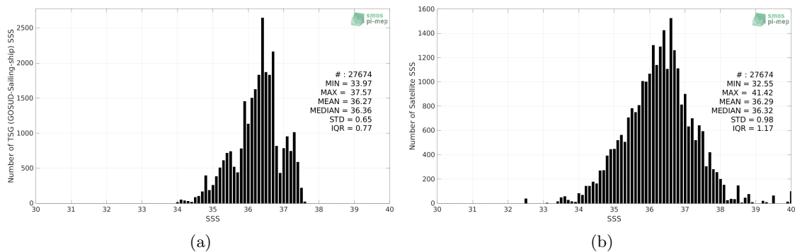
Figure 2: Histograms of SSS from TSG (GOSUD-Sailing-ship) (a) and SMAP SSS L2 v5 - 40 km (RSS) (b) considering all match-up pairs per bins of 0.1 over the Tropical Atlantic Ocean Pi-MEP region and for the full satellite product period.
