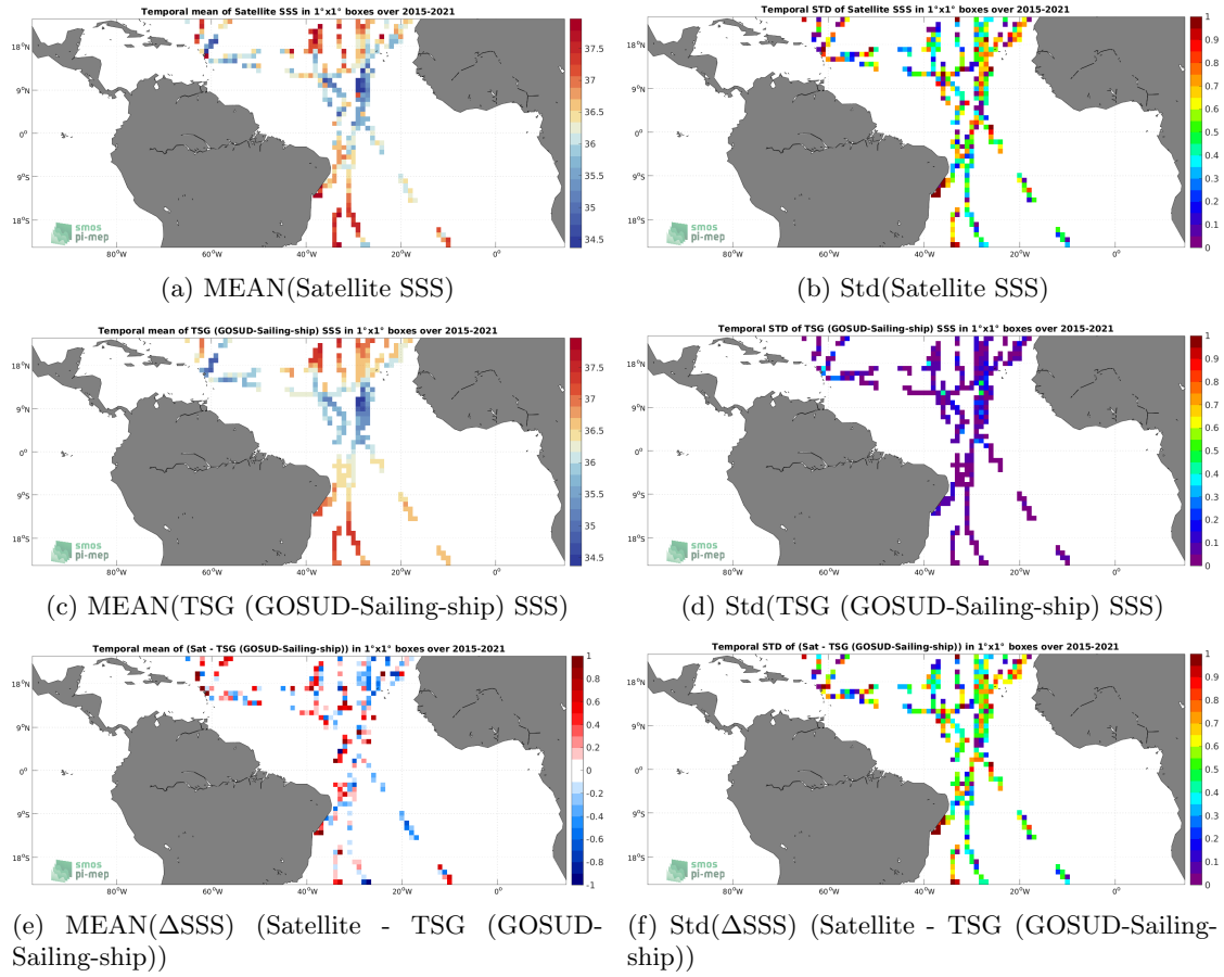
Figure 6: Temporal mean (left) and Std (right) of SSS from SMAP SSS L2 v5 - 40 km (RSS) (top), TSG (GOSUD-Sailing-ship) (middle), and of \Delta SSS (Satellite - TSG (GOSUD-Sailing-ship)). Only match-up pairs are used to generate these maps.
