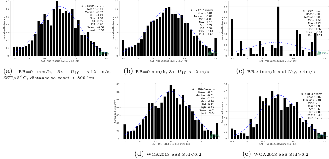
Figure 13: Normalized histogram of \Delta SSS (SMAP SSS L2 v5 - 40 km (RSS) - TSG (GOSUD-Sailing-ship)) for 5 different subdatasets corresponding to: RR=0 mm/h, 3 < U_{10} < 12 m/s, SST > 5°C, distance to coast > 800 km (a), RR=0 mm/h, 3 < U_{10} < 12 m/s (b), RR > 1mm/h and U_{10} < 4 m/s (c), WOA2013 SSS Std < 0.2 (d), WOA2013 SSS Std > 0.2 (e).
