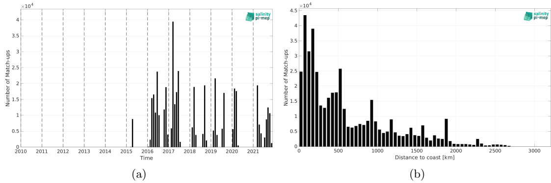
Figure 1: Number of match-ups between TSG (GOSUD-Research-vessel) and SMAP SSS L2 v5 - 40 km (RSS) SSS as a function of time (a) and as function of the distance to coast (b) over the Tropical Atlantic Ocean Pi-MEP region and for the full satellite product period.
