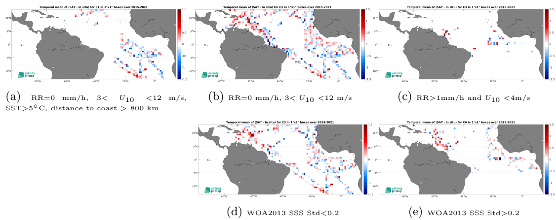
Figure 12: Temporal mean gridded over spatial boxes of size 1^\circ \times 1^\circ of \Delta\text{SSS} (SMAP SSS L2 v5 - 40 km (RSS) - TSG (GOSUD-Research-vessel)) for 5 different subdatasets corresponding to:RR=0 mm/h, 3 < U_{10} < 12 m/s, SST>5°C, distance to coast > 800 km (a), RR=0 mm/h, 3 < U_{10} < 12 m/s (b), RR>1mm/h and U_{10} < 4 m/s (c), WOA2013 SSS Std<0.2 (d), WOA2013 SSS Std>0.2 (e).
