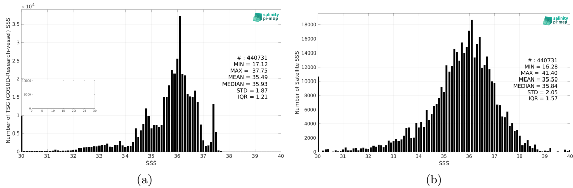
Figure 2: Histograms of SSS from TSG (GOSUD-Research-vessel) (a) and SMAP SSS L2 v5 - 40 km (RSS) (b) considering all match-up pairs per bins of 0.1 over the Tropical Atlantic Ocean Pi-MEP region and for the full satellite product period.
