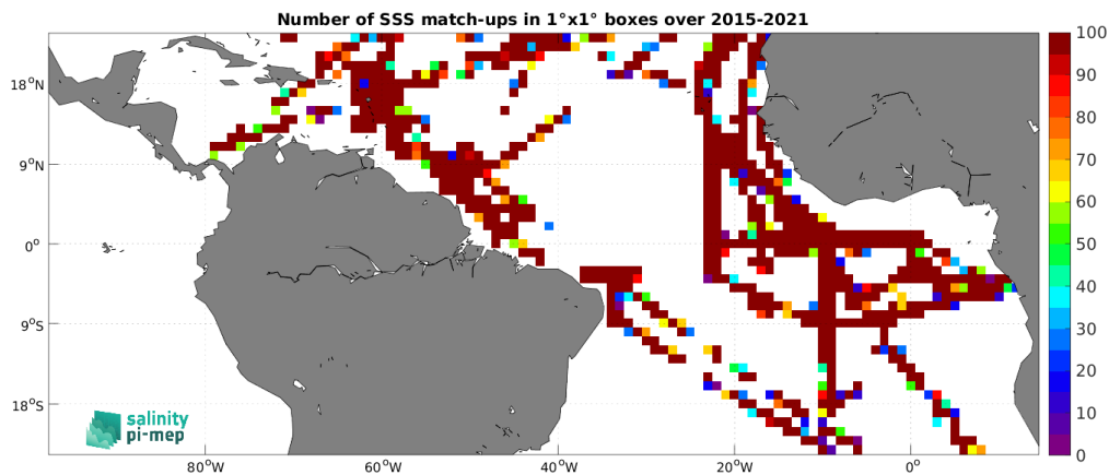
Figure 4: Number of SSS match-ups between TSG (GOSUD-Research-vessel) SSS and the SMAP SSS L2 v5 - 40 km (RSS) SSS product for the Tropical Atlantic Ocean Pi-MEP region over 1^\circ \times 1^\circ boxes and for the full satellite product period.
