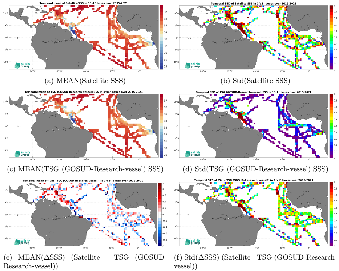
Figure 6: Temporal mean (left) and Std (right) of SSS from SMAP SSS L2 v5 - 40 km (RSS) (top), TSG (GOSUD-Research-vessel) (middle), and of \Delta SSS (Satellite - TSG (GOSUD-Research-vessel)). Only match-up pairs are used to generate these maps.
