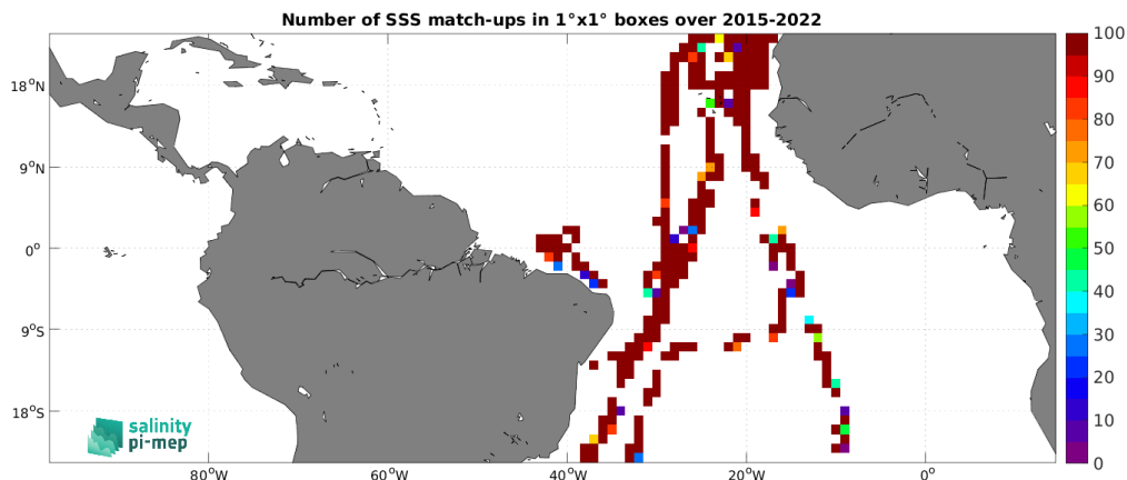
Figure 4: Number of SSS match-ups between TSG (CSIC-UTM) SSS and the SMAP SSS L2 v5 - 40 km (RSS) SSS product for the Tropical Atlantic Ocean Pi-MEP region over 1^\circ \times 1^\circ boxes and for the full satellite product period.
