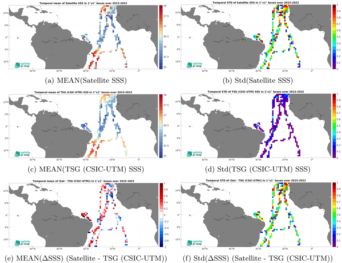
Figure 6: Temporal mean (left) and Std (right) of SSS from SMAP SSS L2 v5 - 40 km (RSS) (top), TSG (CSIC-UTM) (middle), and of \Delta SSS (Satellite - TSG (CSIC-UTM)). Only match-up pairs are used to generate these maps.
