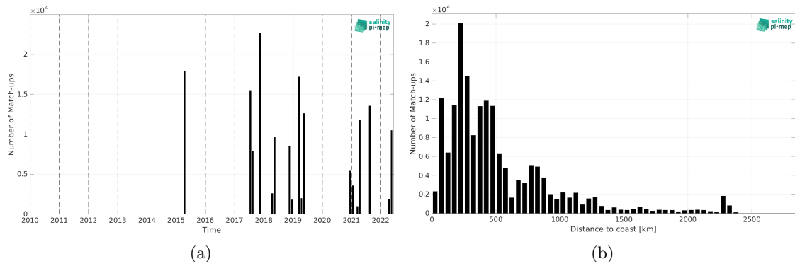
Figure 1: Number of match-ups between TSG (CSIC-UTM) and SMAP SSS L2 v5 - 40 km (RSS) SSS as a function of time (a) and as function of the distance to coast (b) over the Tropical Atlantic Ocean Pi-MEP region and for the full satellite product period.
