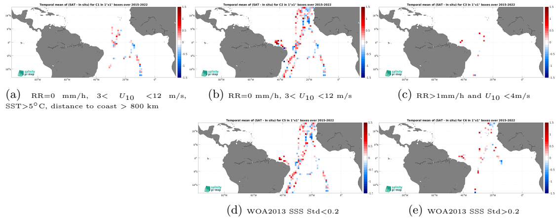
Figure 12: Temporal mean gridded over spatial boxes of size 1^\circ \times 1^\circ of \Delta\text{SSS} (SMAP SSS L2 v5 - 40 km (RSS) - TSG (CSIC-UTM)) for 5 different subdatasets corresponding to:RR=0 mm/h, 3 < U_{10} < 12 m/s, SST >5^\circ\text{C} , distance to coast > 800 km (a), RR=0 mm/h, 3 < U_{10} < 12 m/s (b), RR >1 mm/h and U_{10} < 4 m/s (c), WOA2013 SSS Std <0.2 (d), WOA2013 SSS Std >0.2 (e).
