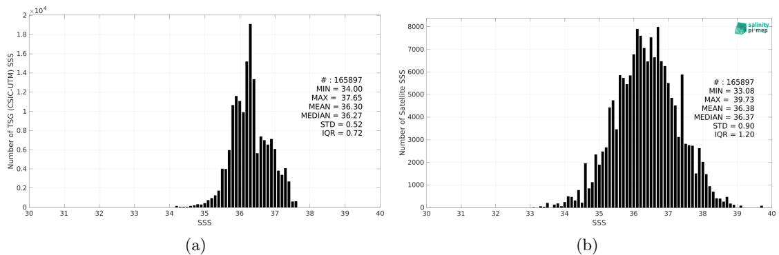
Figure 2: Histograms of SSS from TSG (CSIC-UTM) (a) and SMAP SSS L2 v5 - 40 km (RSS) (b) considering all match-up pairs per bins of 0.1 over the Tropical Atlantic Ocean Pi-MEP region and for the full satellite product period.
