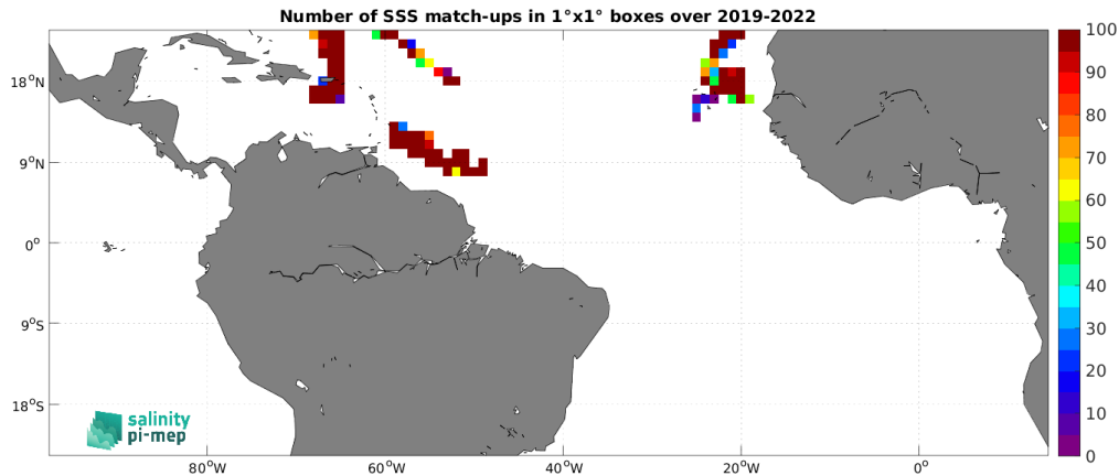
Figure 4: Number of SSS match-ups between Saildrone SSS and the SMAP SSS L2 v5 - 40 km (RSS) SSS product for the Tropical Atlantic Ocean Pi-MEP region over 1^\circ \times 1^\circ boxes and for the full satellite product period.
