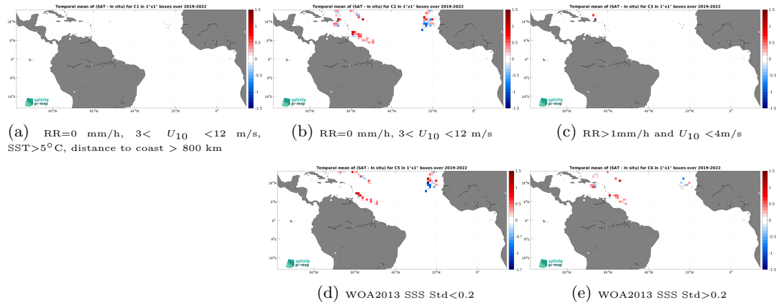
Figure 12: Temporal mean gridded over spatial boxes of size 1^\circ \times 1^\circ of \Delta SSS (SMAP SSS L2 v5 - 40 km (RSS) - Saldrone) for 5 different subdatasets corresponding to:RR=0 mm/h, 3 < U_{10} < 12 m/s, SST >5^\circ\text{C} , distance to coast > 800 km (a), RR=0 mm/h, 3 < U_{10} < 12 m/s (b), RR >1 mm/h and U_{10} < 4 m/s (c), WOA2013 SSS Std <0.2 (d), WOA2013 SSS Std >0.2 (e).
