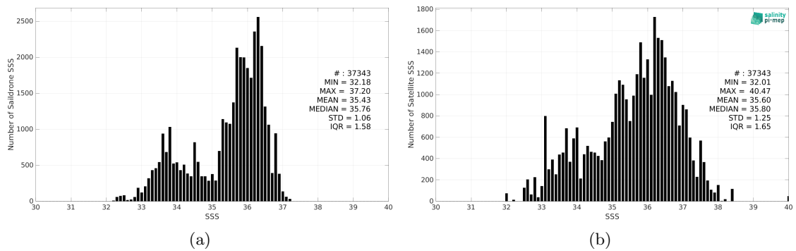
Figure 2: Histograms of SSS from Sairdrone (a) and SMAP SSS L2 v5 - 40 km (RSS) (b) considering all match-up pairs per bins of 0.1 over the Tropical Atlantic Ocean Pi-MEP region and for the full satellite product period.
