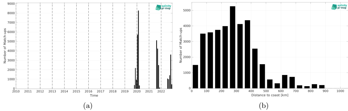
Figure 1: Number of match-ups between Sairdrone and SMAP SSS L2 v5 - 40 km (RSS) SSS as a function of time (a) and as function of the distance to coast (b) over the Tropical Atlantic Ocean Pi-MEP region and for the full satellite product period.
