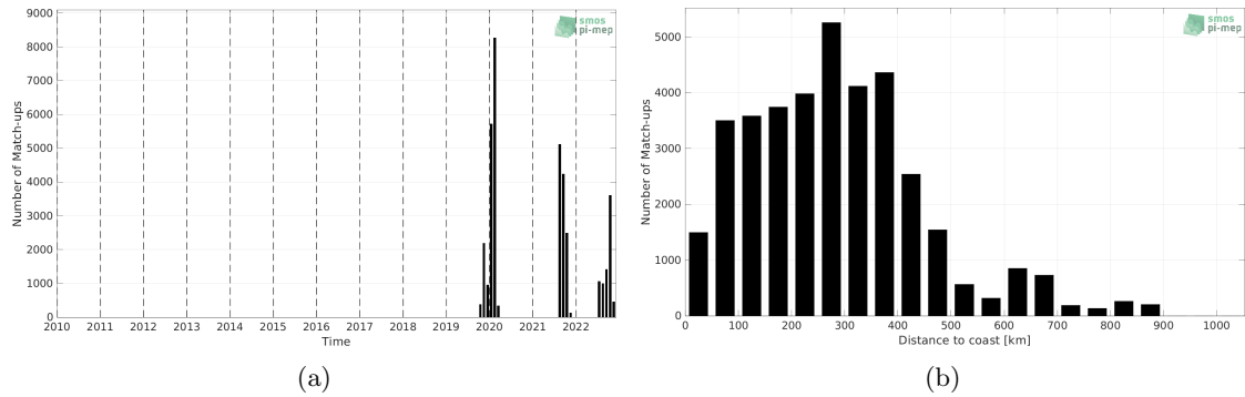
Figure 1: Number of match-ups between Saildrone and SMAP SSS L2 v5 - 40 km (RSS) SSS as a function of time (a) and as function of the distance to coast (b) over the Tropical Atlantic Ocean Pi-MEP region and for the full satellite product period.
