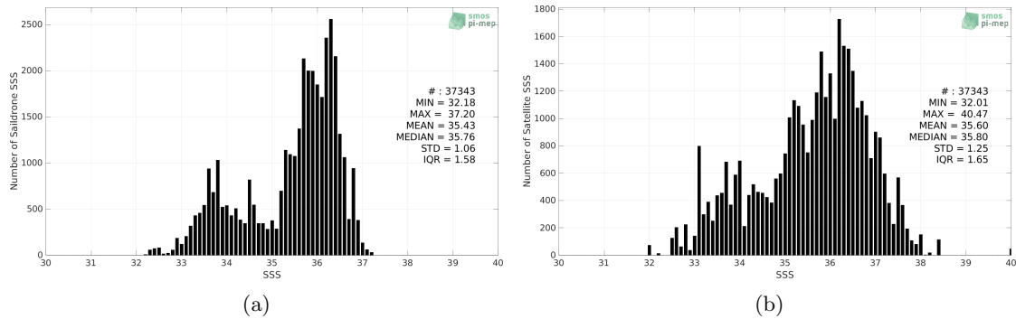
Figure 2: Histograms of SSS from Saildrone (a) and SMAP SSS L2 v5 - 40 km (RSS) (b) considering all match-up pairs per bins of 0.1 over the Tropical Atlantic Ocean Pi-MEP region and for the full satellite product period.
