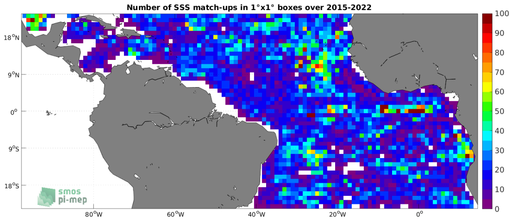
Figure 4: Number of SSS match-ups between Argo SSS and the SMAP SSS L2 v5 - 40 km (RSS) SSS product for the Tropical Atlantic Ocean Pi-MEP region over 1^\circ \times 1^\circ boxes and for the full satellite product period.
