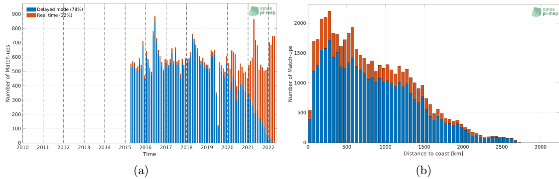
Figure 1: Number of match-ups between Argo and SMAP SSS L2 v5 - 40 km (RSS) SSS as a function of time (a) and as function of the distance to coast (b) over the Tropical Atlantic Ocean Pi-MEP region and for the full satellite product period.
