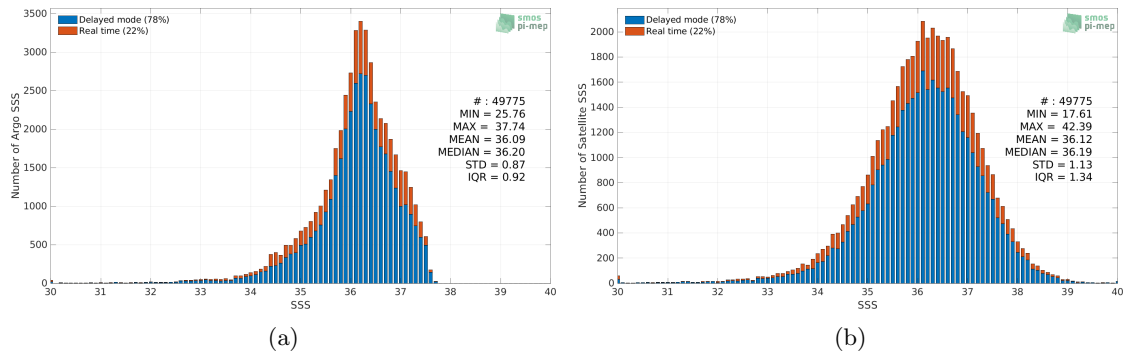
Figure 2: Histograms of SSS from Argo (a) and SMAP SSS L2 v5 - 40 km (RSS) (b) considering all match-up pairs per bins of 0.1 over the Tropical Atlantic Ocean Pi-MEP region and for the full satellite product period.
