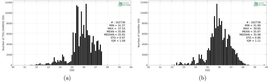
Figure 2: Histograms of SSS from TSG (SAMOS) (a) and SMAP SSS L2 v4 (RSS) (b) considering all match-up pairs per bins of 0.1 over the Tropical Atlantic Ocean Pi-MEP region and for the full satellite product period.
