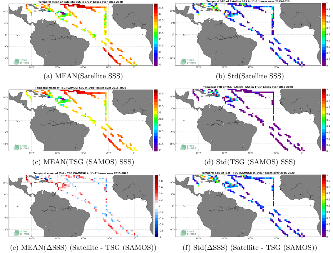
Figure 6: Temporal mean (left) and Std (right) of SSS from SMAP SSS L2 v4 (RSS) (top), TSG (SAMOS) (middle), and of \Delta SSS (Satellite - TSG (SAMOS)). Only match-up pairs are used to generate these maps.
