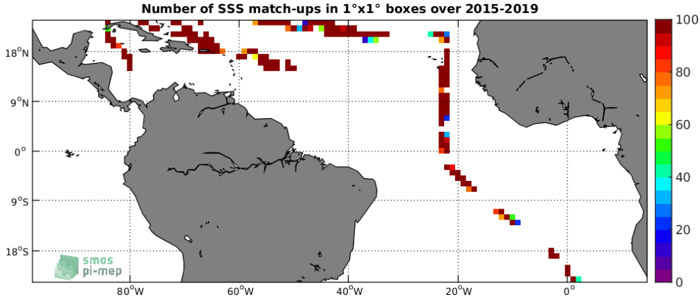
Figure 4: Number of SSS match-ups between TSG-SAMOS SSS and the SMAP-L2-RSS-V4 SSS product for the Tropical Atlantic Ocean Pi-MEP region over 1^\circ \times 1^\circ boxes and for the full satellite product period.
