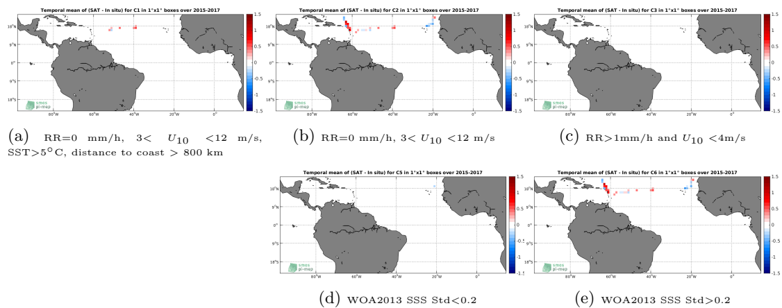
Figure 12: Temporal mean gridded over spatial boxes of size 1^\circ \times 1^\circ of \Delta\text{SSS} (SMAP-L2-RSS-V4 - TSG-GOSUD-Sailing-ship) for 5 different subdatasets corresponding to:RR=0 mm/h, 3 < U_{10} < 12 m/s, SST>5°C, distance to coast > 800 km (a), RR=0 mm/h, 3 < U_{10} < 12 m/s (b), RR>1mm/h and U_{10} < 4 m/s (c), WOA2013 SSS Std<0.2 (d), WOA2013 SSS Std>0.2 (e).
