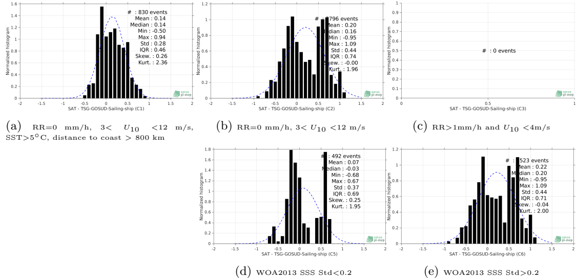
Figure 13: Normalized histogram of \Delta SSS (SMAP-L2-RSS-V4 - TSG-GOSUD-Sailing-ship) for 5 different subdatasets corresponding to: RR=0 mm/h, 3 < U_{10} < 12 m/s, SST > 5°C, distance to coast > 800 km (a), RR=0 mm/h, 3 < U_{10} < 12 m/s (b), RR > 1mm/h and U_{10} < 4 m/s (c), WOA2013 SSS Std < 0.2 (d), WOA2013 SSS Std > 0.2 (e).
