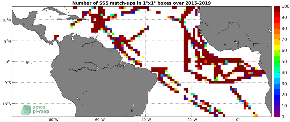
Figure 4: Number of SSS match-ups between TSG (GOSUD-Research-vessel) SSS and the SMAP SSS L2 v4 (RSS) SSS product for the Tropical Atlantic Ocean Pi-MEP region over 1^\circ \times 1^\circ boxes and for the full satellite product period.
