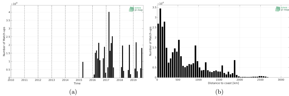
Figure 1: Number of match-ups between TSG (GOSUD-Research-vessel) and SMAP SSS L2 v4 (RSS) SSS as a function of time (a) and as function of the distance to coast (b) over the Tropical Atlantic Ocean Pi-MEP region and for the full satellite product period.
