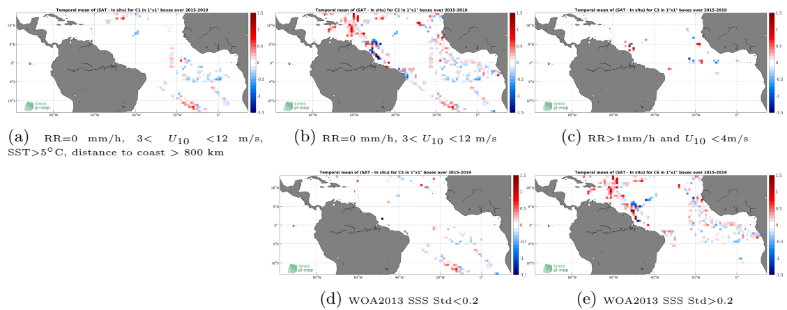
Figure 12: Temporal mean gridded over spatial boxes of size 1°x1° of \Delta SSS (SMAP SSS L2 v4 (RSS) - TSG (GOSUD-Research-vessel)) for 5 different subdatasets corresponding to:RR=0 mm/h, 3 < U_{10} < 12 m/s, SST>5°C, distance to coast > 800 km (a), RR=0 mm/h, 3 < U_{10} < 12 m/s (b), RR>1mm/h and U_{10} < 4 m/s (c), WOA2013 SSS Std<0.2 (d), WOA2013 SSS Std>0.2 (e).
