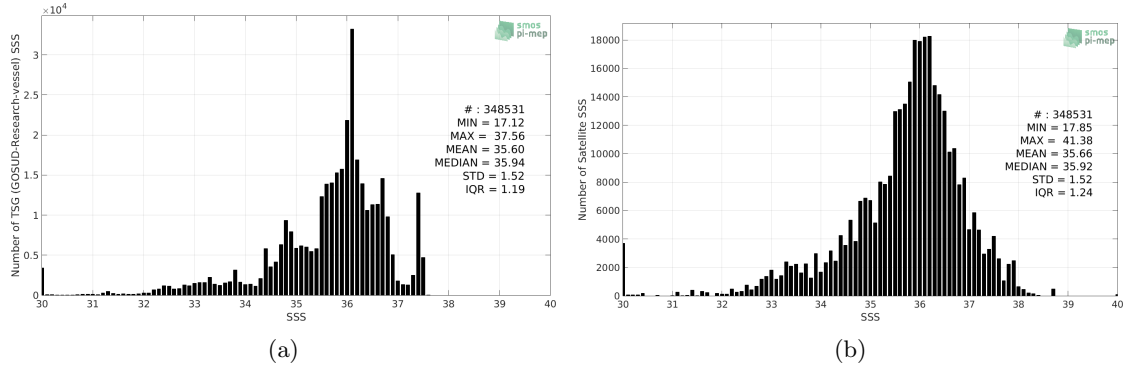
Figure 2: Histograms of SSS from TSG (GOSUD-Research-vessel) (a) and SMAP SSS L2 v4 (RSS) (b) considering all match-up pairs per bins of 0.1 over the Tropical Atlantic Ocean Pi-MEP region and for the full satellite product period.
