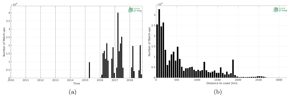
Figure 1: Number of match-ups between TSG-GOSUD-Research-vessel and SMAP-L2-RSS-V4 SSS as a function of time (a) and as function of the distance to coast (b) over the Tropical Atlantic Ocean Pi-MEP region and for the full satellite product period.
