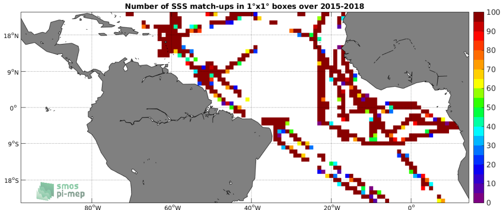
Figure 4: Number of SSS match-ups between TSG-GOSUD-Research-vessel SSS and the SMAP-L2-RSS-V4 SSS product for the Tropical Atlantic Ocean Pi-MEP region over 1^\circ \times 1^\circ boxes and for the full satellite product period.
