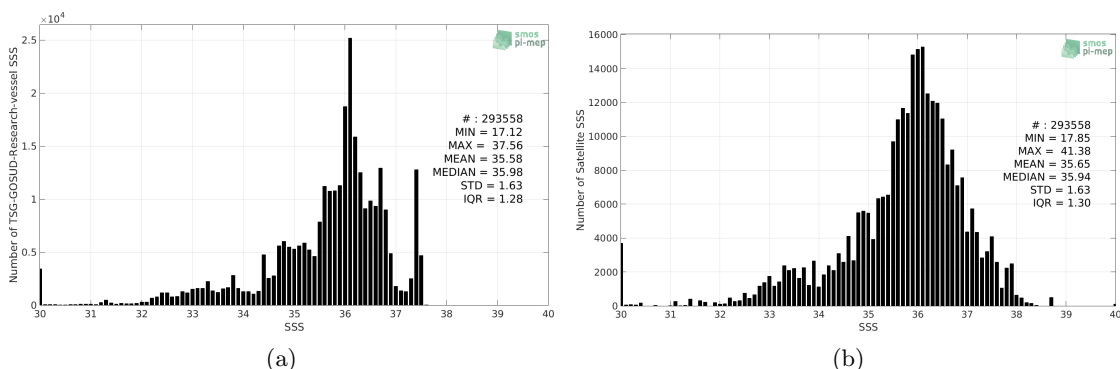
Figure 2: Histograms of SSS from TSG-GOSUD-Research-vessel (a) and SMAP-L2-RSS-V4 (b) considering all match-up pairs per bins of 0.1 over the Tropical Atlantic Ocean Pi-MEP region and for the full satellite product period.
