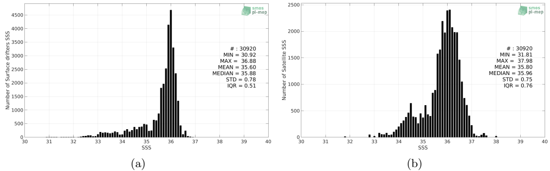
Figure 2: Histograms of SSS from Surface drifters (a) and SMAP SSS L2 v4 (RSS) (b) considering all match-up pairs per bins of 0.1 over the Tropical Atlantic Ocean Pi-MEP region and for the full satellite product period.
