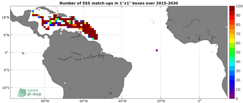
Figure 3: Number of SSS match-ups between Surface drifters SSS and the SMAP SSS L2 v4 (RSS) SSS product for the Tropical Atlantic Ocean Pi-MEP region over 1^\circ \times 1^\circ boxes and for the full satellite product period.
