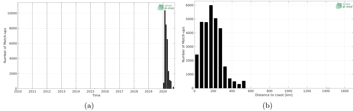
Figure 1: Number of match-ups between Surface drifters and SMAP SSS L2 v4 (RSS) SSS as a function of time (a) and as function of the distance to coast (b) over the Tropical Atlantic Ocean Pi-MEP region and for the full satellite product period.
