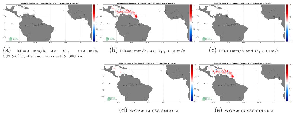
Figure 11: Temporal mean gridded over spatial boxes of size 1^\circ \times 1^\circ of \Delta SSS (SMAP SSS L2 v4 (RSS) - Surface drifters) for 5 different subdatasets corresponding to:RR=0 mm/h, 3 < U_{10} < 12 m/s, SST>5°C, distance to coast > 800 km (a), RR=0 mm/h, 3 < U_{10} < 12 m/s (b), RR>1mm/h and U_{10} < 4 m/s (c), WOA2013 SSS Std<0.2 (d), WOA2013 SSS Std>0.2 (e).
