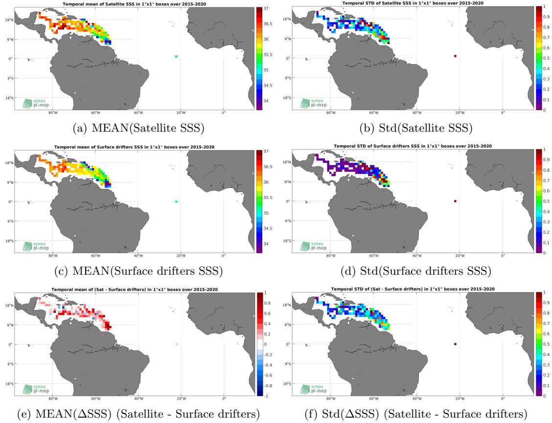
Figure 5: Temporal mean (left) and Std (right) of SSS from SMAP SSS L2 v4 (RSS) (top), Surface drifters (middle), and of \Delta SSS (Satellite - Surface drifters). Only match-up pairs are used to generate these maps.
