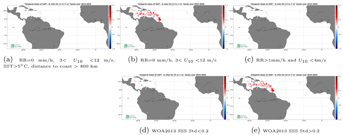
Figure 11: Temporal mean gridded over spatial boxes of size 1^\circ \times 1^\circ of \Delta SSS (SMAP SSS L2 v4 (RSS) - Surface drifters) for 5 different subdatasets corresponding to: RR=0 mm/h, 3 < U_{10} < 12 m/s, SST > 5°C, distance to coast > 800 km (a), RR=0 mm/h, 3 < U_{10} < 12 m/s (b), RR > 1mm/h and U_{10} < 4 m/s (c), WOA2013 SSS Std < 0.2 (d), WOA2013 SSS Std > 0.2 (e).
