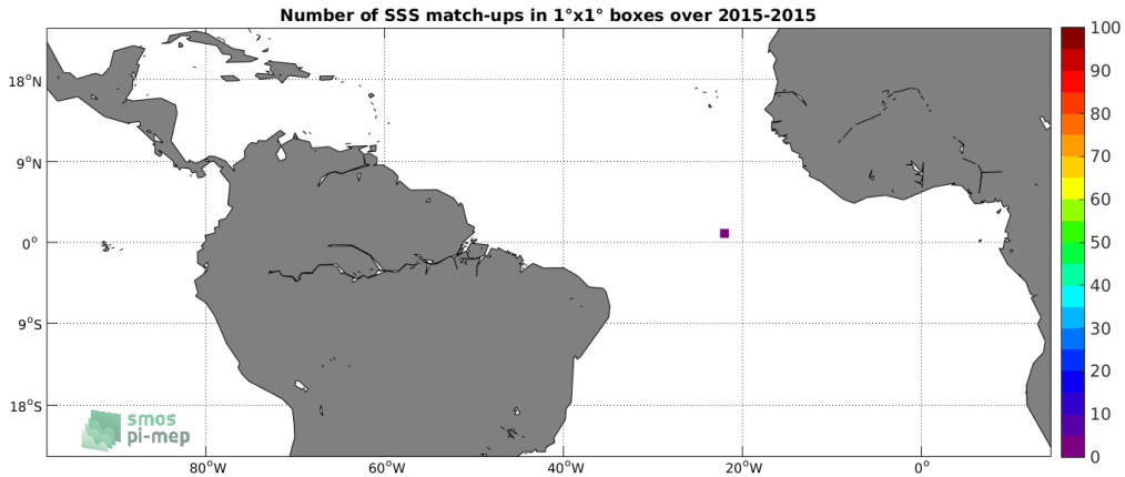
Figure 3: Number of SSS match-ups between Surface drifters SSS and the SMAP SSS L2 v4 (RSS) SSS product for the Tropical Atlantic Ocean Pi-MEP region over 1°x1° boxes and for the full satellite product period.
