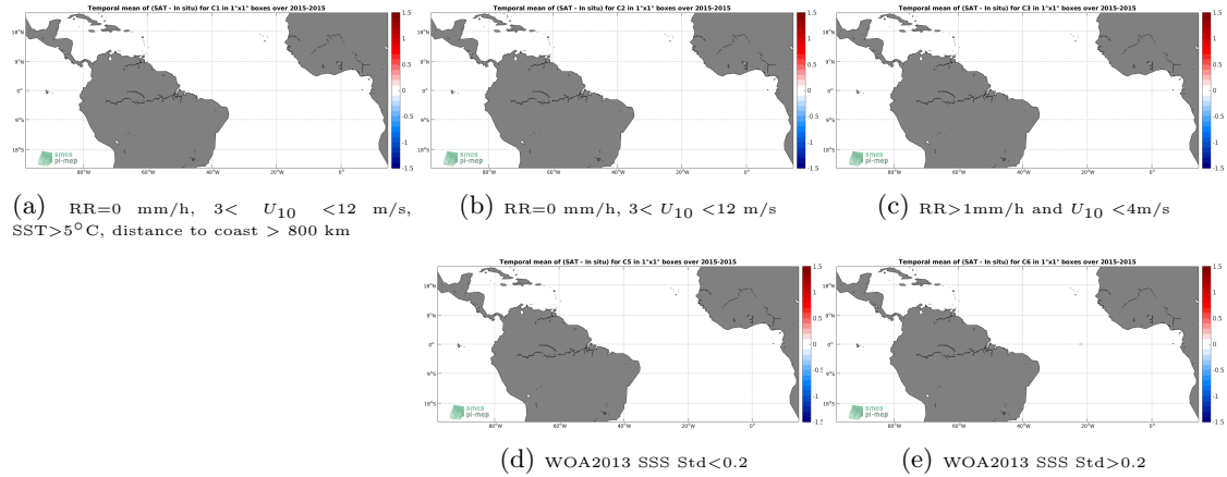
Figure 11: Temporal mean gridded over spatial boxes of size 1^{\circ}\times 1^{\circ} of \Delta\text{SSS} (SMAP SSS L2 v4 (RSS) - Surface drifters) for 5 different subdatasets corresponding to:RR=0 mm/h, 3 < U_{10} < 12 m/s, SST >5^{\circ}\text{C} , distance to coast > 800 km (a), RR=0 mm/h, 3 < U_{10} < 12 m/s (b), RR >1 mm/h and U_{10} < 4 m/s (c), WOA2013 SSS Std <0.2 (d), WOA2013 SSS Std >0.2 (e).
