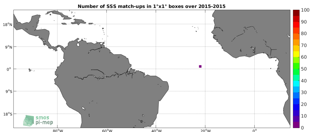
Figure 3: Number of SSS match-ups between Surface drifters SSS and the SMAP-L2-RSS-V4 SSS product for the Tropical Atlantic Ocean Pi-MEP region over 1°x1° boxes and for the full satellite product period.
