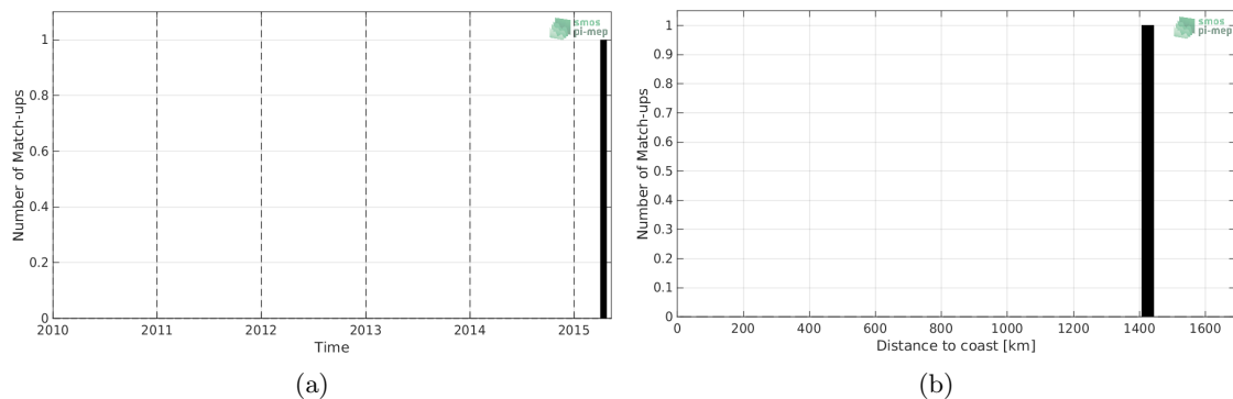
Figure 1: Number of match-ups between Surface drifters and SMAP-L2-RSS-V4 SSS as a function of time (a) and as function of the distance to coast (b) over the Tropical Atlantic Ocean Pi-MEP region and for the full satellite product period.
