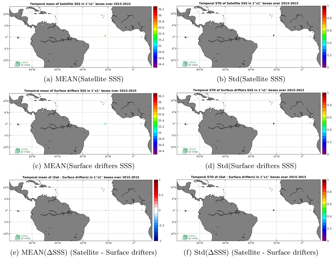
Figure 5: Temporal mean (left) and Std (right) of SSS from SMAP-L2-RSS-V4 (top), Surface drifters (middle), and of \Delta SSS (Satellite - Surface drifters). Only match-up pairs are used to generate these maps.
