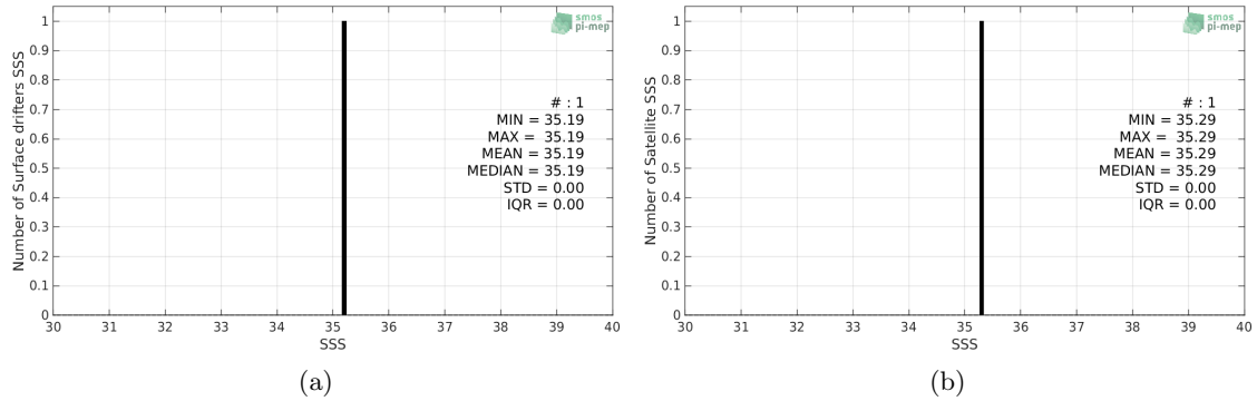
Figure 2: Histograms of SSS from Surface drifters (a) and SMAP-L2-RSS-V4 (b) considering all match-up pairs per bins of 0.1 over the Tropical Atlantic Ocean Pi-MEP region and for the full satellite product period.
