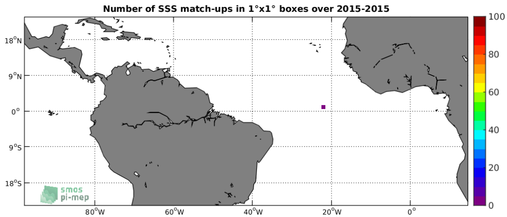
Figure 3: Number of SSS match-ups between Surface drifters SSS and the SMAP-L2-RSS-V4 SSS product for the Tropical Atlantic Ocean Pi-MEP region over 1^\circ \times 1^\circ boxes and for the full satellite product period.
